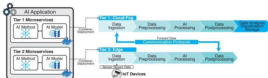
Figure 1: Video surveillance application implemented in a two-tier architecture.
