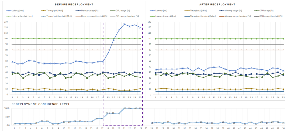
Figure 6: Monitoring data comparison before and after the redeployment process. The MDP method's probabilistic assurances are provided as confidence levels and are used to make a decision on redeployment. When such decision is taken the MDP decision-making method is used to choose a new deployment option based on the available pool of resources.
