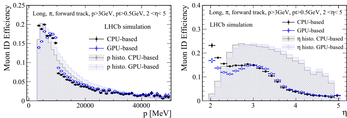
Fig. 10 Efficiency to falsely identify true pions reconstructed as long muon tracks as muons as function of the pion momentum and pseudorapidity
