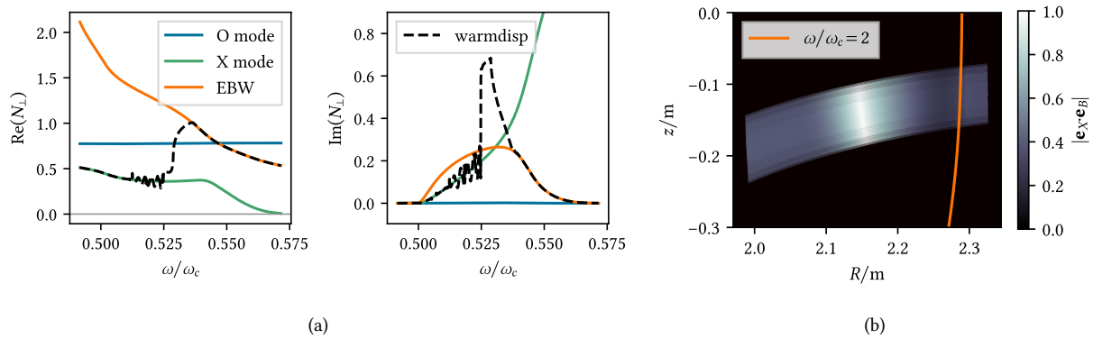
Figure 1: fig. 1a, dispersion curves with the standard warmdisp solver (dashed) exhibiting unstable behaviour and jumping to the wrong branch; the solid lines are obtained by hotdisp . fig. 1b X-B conversion region visualised by a beam and the coupling strength between the mode polarisations vectors \mathbf{e}_X \cdot \mathbf{e}_B , obtained with hotdisp . The latter allows detecting mode conversion events and, if combined with a ray-splitting method [8], could be used to study O-X-B heating schemes [9] or X-B conversion during the plasma start-up. This possibility is currently being explored.
