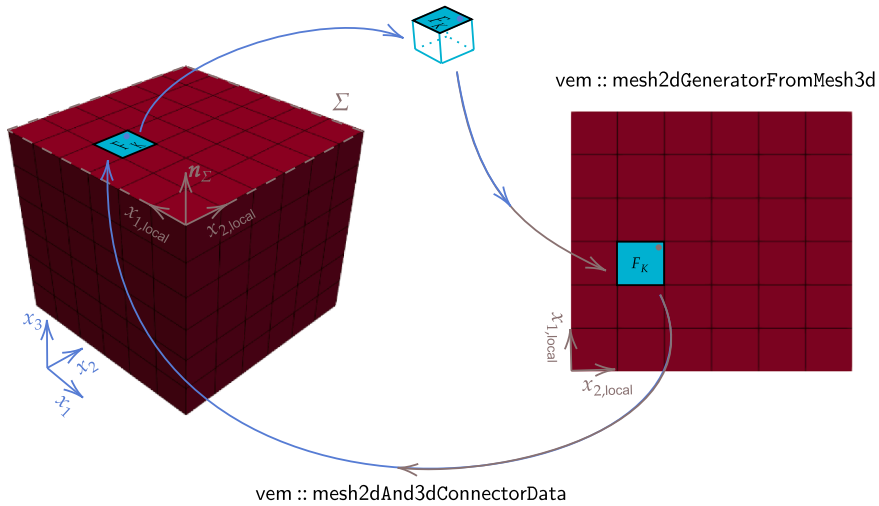
Fig. 2. Diagram for creation of a 2D mesh from the surface of a 3D mesh, the bijective map between entities in 3D and 2D is shown with blue and grey arrows. (For interpretation of the references to colour in this figure legend, the reader is referred to the web version of this article.)
