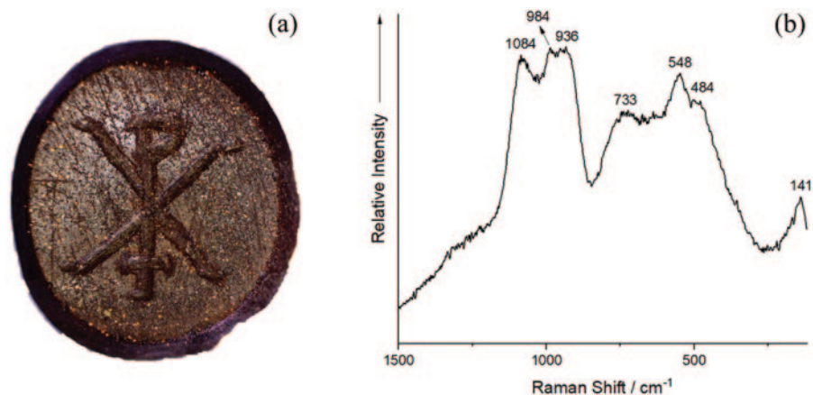
Fig. 1. – Identification of the study case: (a) sample Inv. No. 26271; (b) the relative Raman spectrum. Acquisition parameters: 532 nm source, 20 cycles/30 seconds each, Optical Microscopy object 80 \times corresponding to 20 \mu m spot. © Direzione Regionale Musei del Friuli Venezia Giulia - Museo Archeologico Nazionale di Aquileia.
