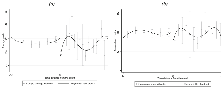
Fig. 2 Average grades and accumulated credits around the 60-min cut-off. Note 0 corresponds to the 60-min threshold. CIs are estimated using the IMSE optimal number of bins for equally spaced bins on the running variable support
