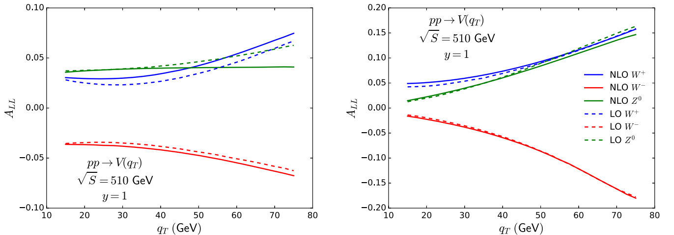
FIG. 11. Longitudinal double spin asymmetries in on-shell weak boson V production at rapidities y = 0 and y = 1 .
