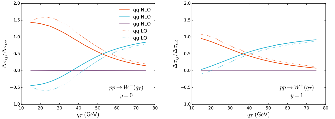
FIG. 10. Subchannel contributions to on-shell W^+ boson production with rapidities y = 0 and y = 1 . Both NLO and LO decompositions are given.
