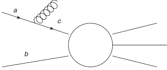
FIG. 2. Schematic of the parton emission processes.
