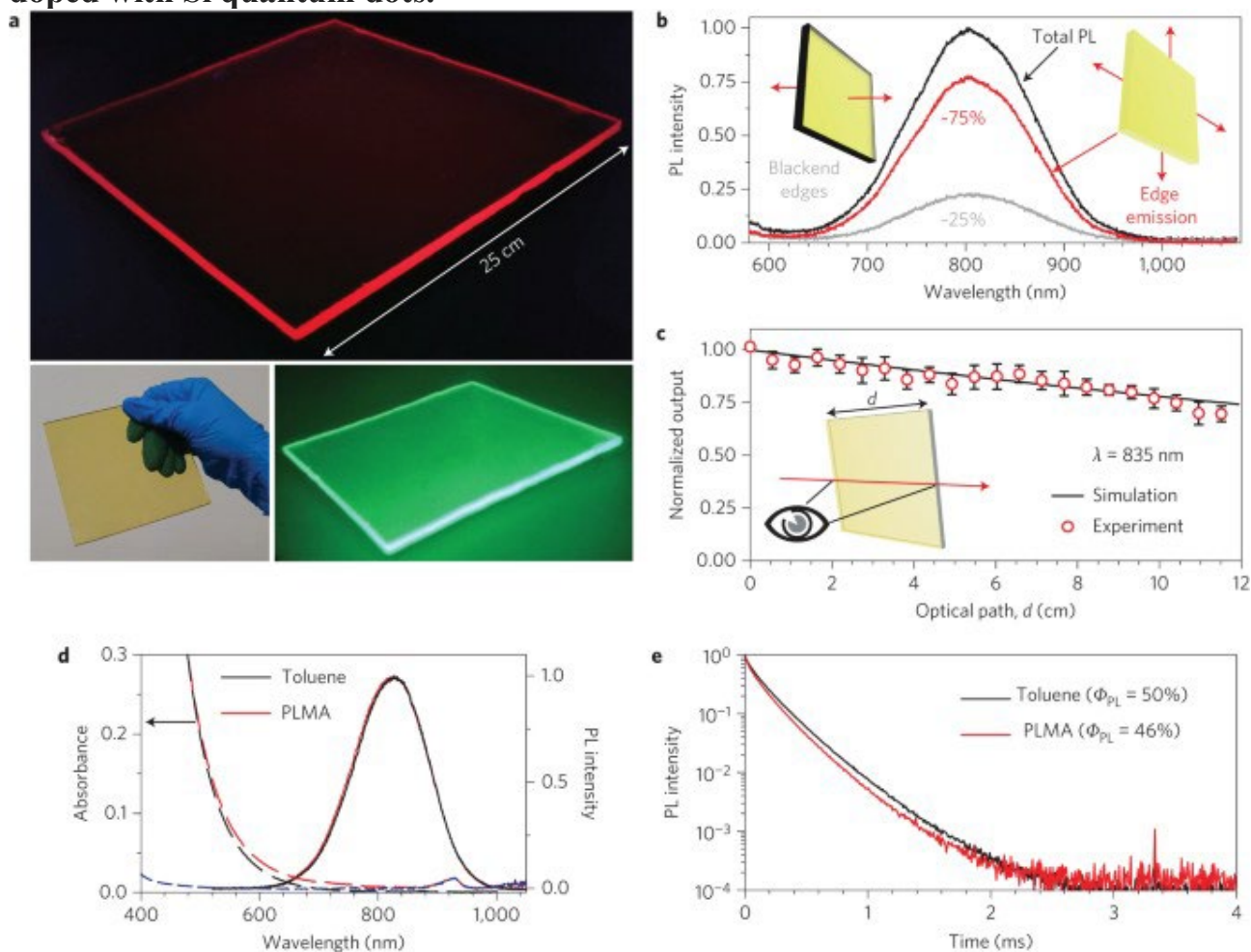
Figure 2: Large-area LSCs based on mass polymerized nanocomposite waveguides doped with Si quantum dots.
