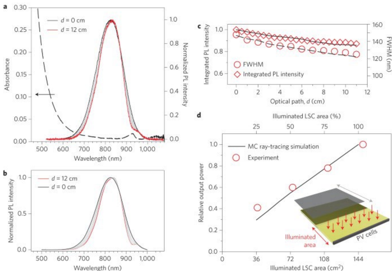
a , Absorption spectrum of the QD-LSC (0.09 wt% Si quantum dots, dimensions of 12 cm × 12 cm × 0.26 cm, dashed line) and normalized photoluminescence spectra collected at the edge of the LSC when the excitation spot is located at distances d = 0 cm or d = 12 cm from the edge. The spectra at intermediate d values are reported as grey curves. b , Photoluminescence (PL) spectra versus d calculated through Monte Carlo (MC) ray-tracing simulation. c , Full-width at half-maximum (FWHM) and integrated intensity of the experimental and simulated luminescence spectra versus d . d , Relative optical output power measured from one LSC edge as a function of device area illuminated by a calibrated solar simulator. The trend obtained through Monte Carlo simulation of an ideal LSC with no scattering/reabsorption losses and embedding emitters with the same quantum efficiency as the Si quantum dots ( \Phi_{\text{PL}} = 46\% ) is reported as a black curve.
