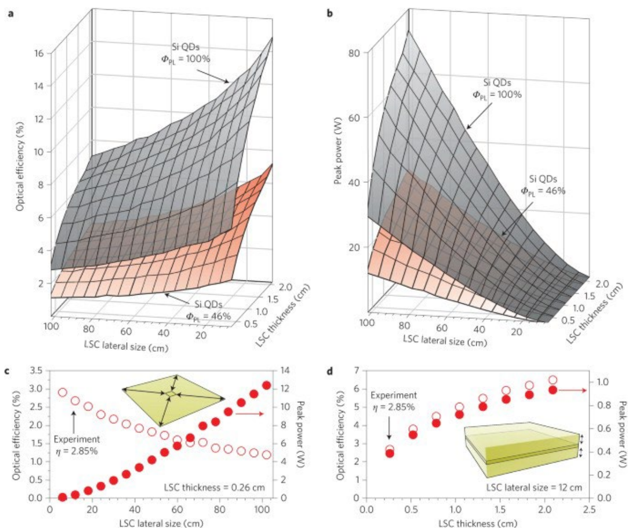
a,b , Three-dimensional plots of optical power efficiency \eta ( a ) and peak power output (at 1.5 AM Global irradiance) calculated through Monte Carlo ray-tracing simulations ( b ) as a function of LSC area and thickness (shaded in red for \Phi_{PL} = 46\% and in grey for \Phi_{PL} = 100\% ). c,d , Theoretical trends of \eta (open circles) and peak power output (filled red circles) for square LSCs with the experimental thickness (0.26 cm) and increasing lateral size ( c ) and the experimental area (lateral size 12 \times 12 \text{ cm}^2 ) and increasing slab thickness ( d ) (in both cases \Phi_{PL} = 46\% ).
