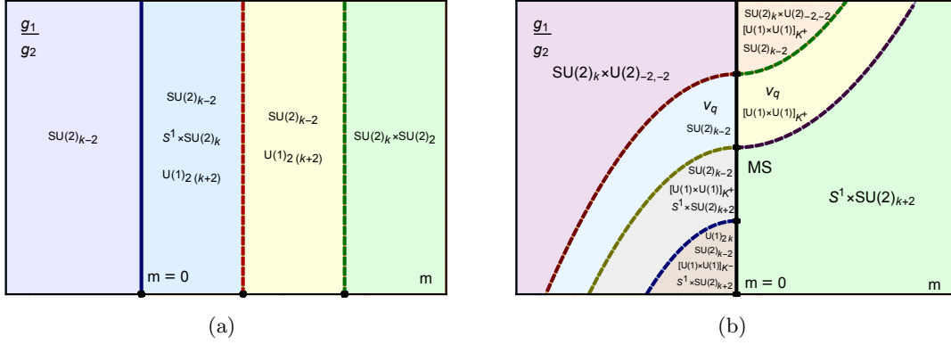
Figure 8. Phase diagram for the SU(2)_k \times SU(2)_0 quiver (a) and for the SU(2)_k adjoint QCD (b).
