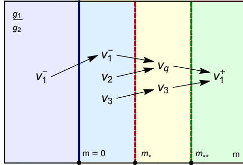
Figure 2. Structure of the phase diagrams of the SU(2)_{k_1} \times SU(2)_{k_2} quivers and, as will be clear later, the SU(2)_{k_1} \times U(2)_{k_2, k_3} quivers with either k_1, k_2 > 1 , or k_1 = 0, k_2 > 1 . Dashed lines correspond to the second order phase transitions, while the solid line is the wall. Supersymmetric vacua at each phase are indicated.
