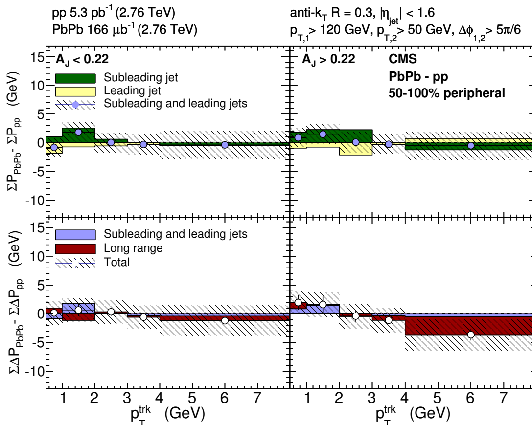
Figure 12. Modifications of jet-track correlated p_T^{\text{trk}} in peripheral PbPb collisions with respect to the pp reference data, integrated over |\Delta\phi| < \pi/2 and |\Delta\eta| < 2.5 . Top row: subleading and leading jet peaks PbPb-pp. Bottom row: relative contributions from jet peaks and two-dimensional asymmetry to the double difference PbPb-pp, subleading-leading in total hemisphere p_T^{\text{trk}} . Statistical uncertainties are shown with vertical bars, and systematic uncertainties are shown with shaded boxes.
