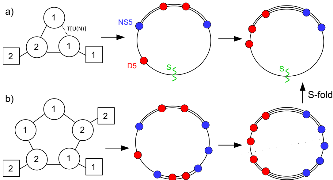
Figure 9. a) An \mathcal{S} -flip quiver and its brane realization. On the right: a canonical brane realization after Hanany-Witten moves, giving the quiver data \rho_1 = (1, 1, 0) , \rho_2 = (1, 1) , N = 3 (number of D3s at the top). b) The parent circular quiver and its brane realization. On the right: the same brane configuration after Hanany-Witten moves, and the quotient by \mathcal{S} .
