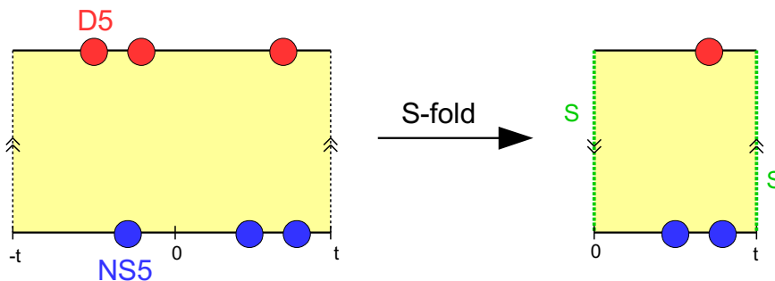
Figure 8. An example of \mathcal{S} -folding. The resulting \mathcal{S} -flip solution has an \mathcal{S} monodromy cut (green dashed line).
