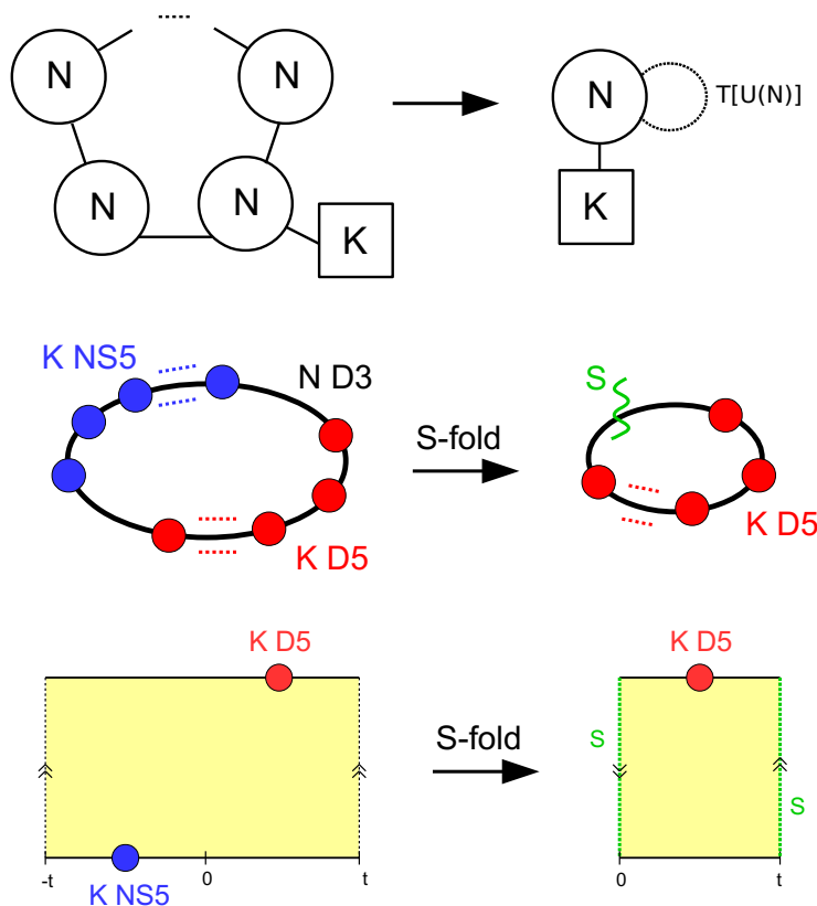
Figure 11. \mathcal{S} -quotient leading to the pure D5 theory. The double cover theory has K U(N) nodes and K fundamental hypermultiplets in one node. The double cover supergravity solution has single stacks of K D5s and K NS5s.
