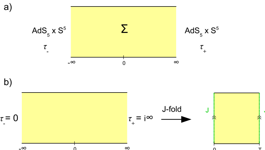
Figure 1. a) Picture of \Sigma (yellow strip) for the Janus solution with asymptotic axio-dilaton values \tau_{\pm} . b) J -folding of the extremal Janus solution. This involves an SL(2, \mathbb{R}) transformation before taking the J -fold quotient. The resulting solution has a cut (green) with J monodromy.
