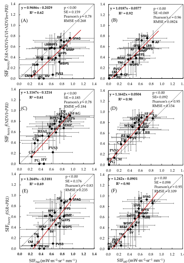
Figure 7. Scatterplots of the best performing fuzzy logic model outputs (SIF fuzzy ) and actual SIFs (SIF 760 and SIF 687 ) were determined based on HyPlant airborne data. (A,B) SIF fuzzy expressed by f(NDVI+EVI+NDVI_{re}+SR+PRI) under model C6; (C,D) SIF fuzzy expressed by f(NDVI+PRI) under
