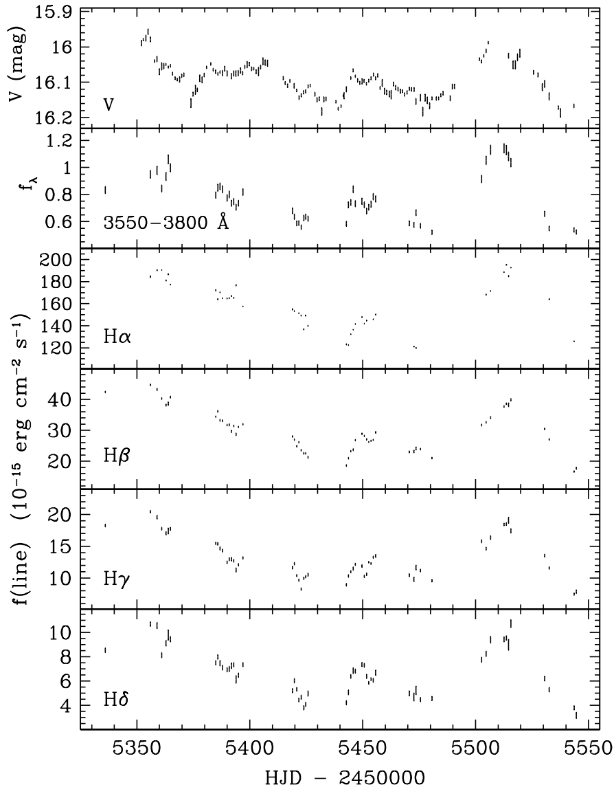
FIG. 5.— Light curves of the V -band continuum, the spectroscopic continuum over 3550–3800 Å (in units of 10^{-15} erg \text{cm}^{-2} Å ^{-1} ), and the H\alpha , H\beta , H\gamma , and H\delta emission lines. The displayed V -band light curve is the “condensed” version in which measurements separated by less than 5 hr have been averaged together giving a single data point per night. The 3550–3800 Å continuum light-curve points are plotted with error bars of \pm 3\% as a rough approximation of the uncertainties from the spectral scaling procedure and slit losses, since these errors dominate over photon-counting uncertainties.
