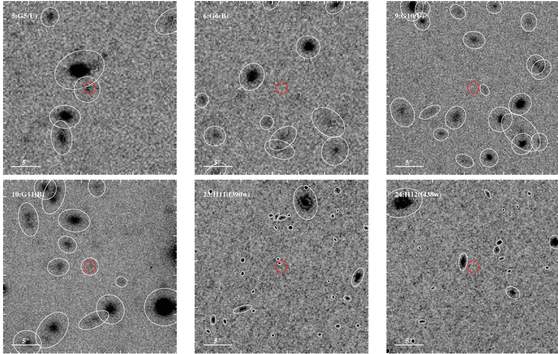
Figure 8. Images in the bluest available filters of the six quasar fields with candidate DLA galaxies at close impact parameters. Each panel shows a 30 arcsec \times 30 arcsec region centred at the DLA position, which is marked by a red circle. The detected sources are marked with white ellipses, which represent the Kron apertures used for photometry.
