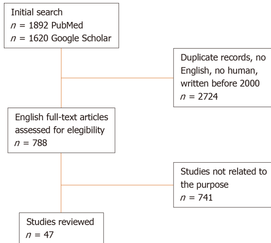
Figure 1 Literature research.
