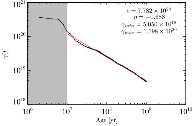
Figure B1. Fit of a simple power-law approximation ( 1/\Upsilon \propto t^{-\xi} , red) for the light to mass ratio 1/\Upsilon(t) , compared to the results of a STARBURST99 calculation of \Upsilon with a Kroupa IMF, Padova+AGB stellar tracks, Lej+SMI stellar atmospheres and solar metallicity (black). The greyed out region corresponds to populations younger than 10 Myr, for which the fit is poor.
