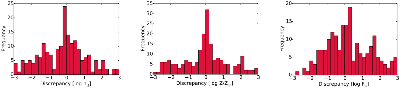
Figure A2. Same as Fig. A1, but including systematic errors on the ion column densities.
