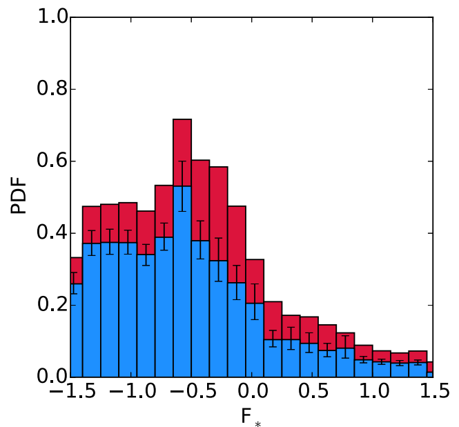
Figure 11. Same as Fig. 3, but for the posterior PDF of F_* in the dust model. The majority of LLSs, especially at z > 2 , are characterized by a low dust content with F_* \lesssim 0 .
