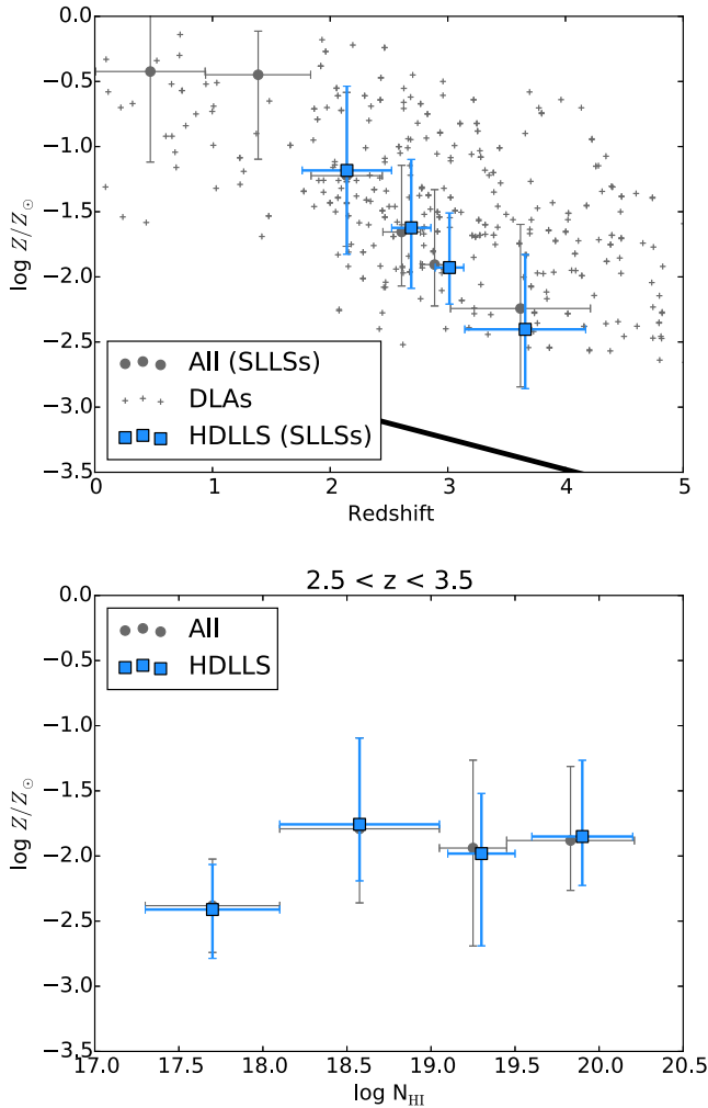
Figure 15. Top: redshift evolution of the metallicity for all the LLSs with \log N_{\text{H I}} \geq 19 in our sample (grey circles), and for the subset from the HD-LLS survey (blue squares). Data points and their associated error bars represent the median and the 25th/75th percentiles of the composite posterior PDFs in redshift bins that are chosen to contain at least 25 LLSs each. Metallicity measurements for individual DLAs from the literature are also superimposed (crosses). The black line marks the median IGM metallicity (Simcoe 2011). A clear trend with redshift is visible. Bottom: dependency on the metallicity as a function of column density for all the LLSs at z \sim 2.5\text{--}3.5 (grey circles) and the HD-LLS subset (blue squares), showing tentative evidence that lowest column density systems are the most metal poor.
