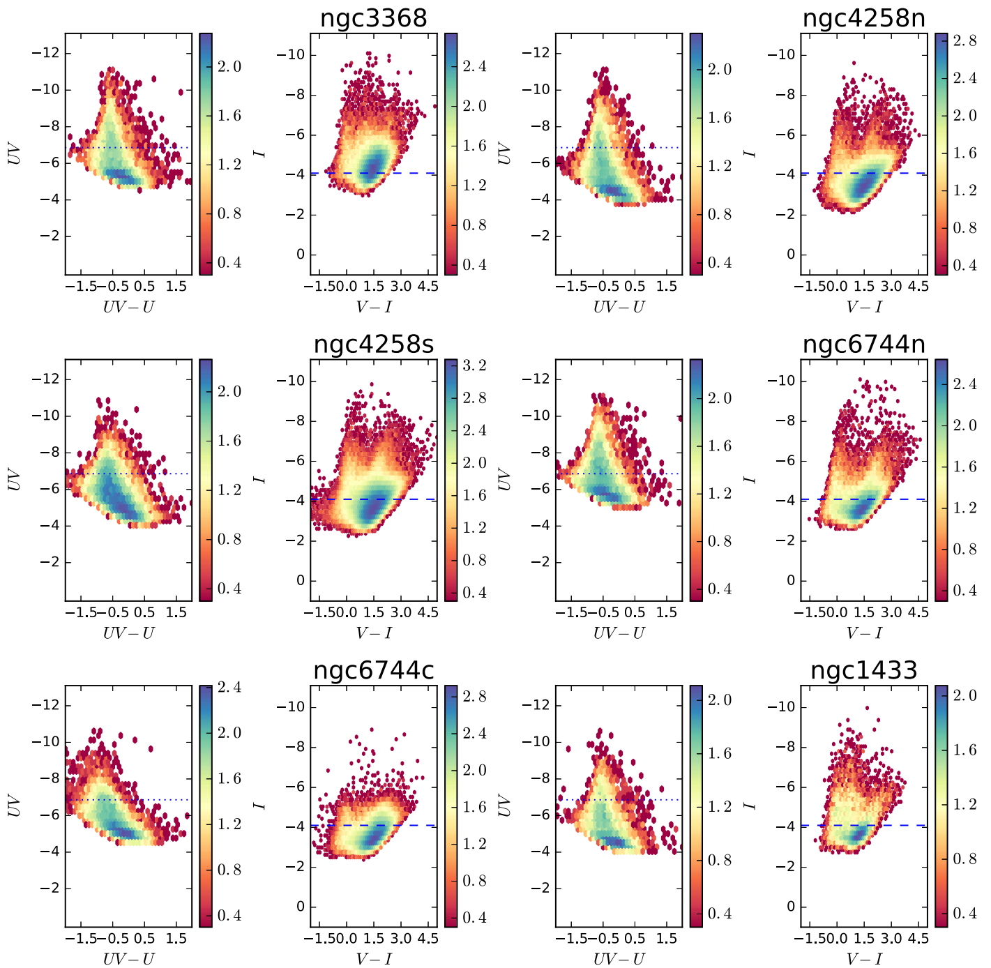
Figure 13. Same as Figure 5, but for the galaxies NGC 3368, NGC 4258 (north and south), NGC 6744 (north and Center), and NFC 1433.
