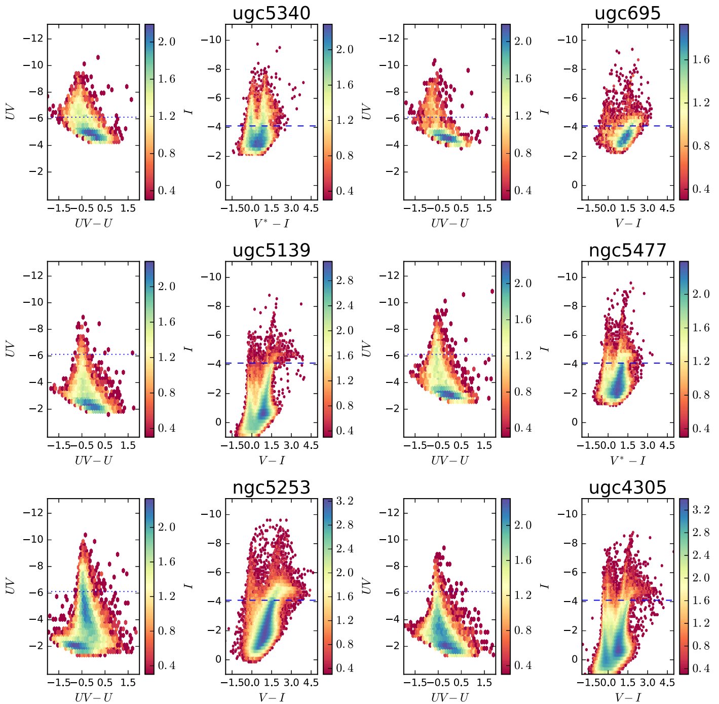
Figure 6. Same as Figure 5, but for the galaxies UGC 5340, UGC 695, UGC 5139, NGC 5477, NGC 5253, UGC 4305. Magnitudes marked as V^* refer to the filter F606W, instead of F555W.
