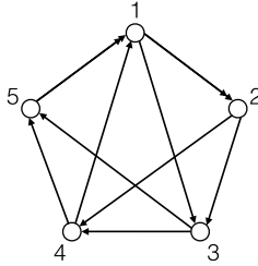
Fig. 4. Quiver of the dP_2^{(I)} model.
