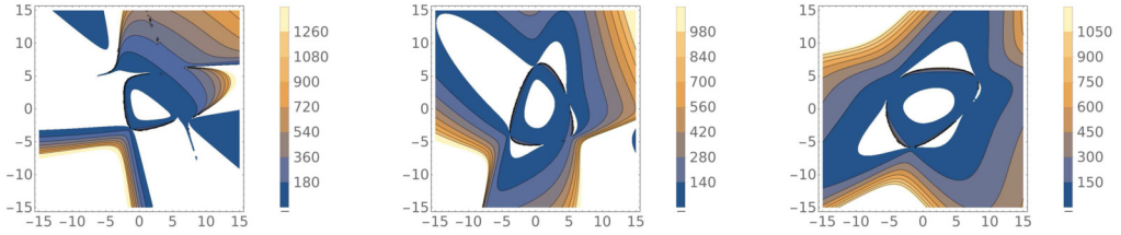
Fig. 11. Central charge of dP_2 on \Sigma = S^2 for different values of the integer fluxes. We plot the regions of fluxes b_i in which the central charge assumes a positive value. In the first case we have fixed b_1 = x , b_2 = y and b_3 = b_4 = 0 . In the second case we have fixed b_3 = x and b_4 = y and b_1 = b_2 = 0 . In the third case we have fixed b_2 = x , b_3 = y and b_1 = b_4 = 0 .
