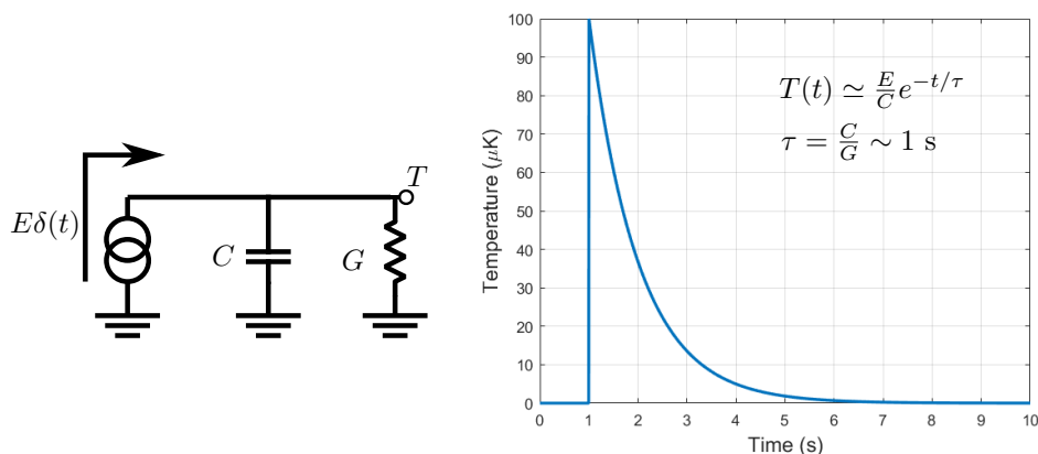
Figure 3.4: Equivalent electric circuit simulating the bolometer response. Ground reference is the thermal bath, C the crystal thermal capacitance, G the thermal conductivity to the thermal bath and the \delta(t) current source represents the thermal power injected by an interacting particle. A typical temperature pulse as a function of time is depicted on the right.
