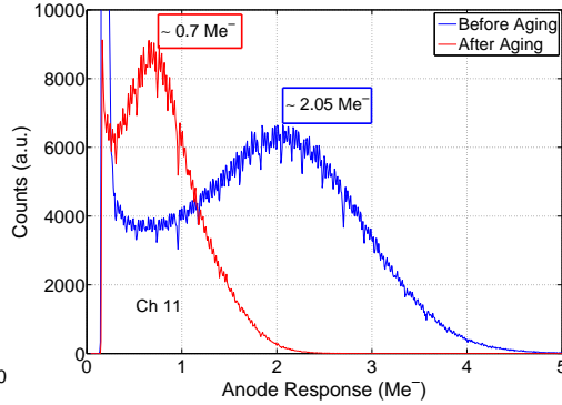
Figure 2.38: Single photon spectra acquired in the most illuminated pixel (channel 11) before and after the aging.
