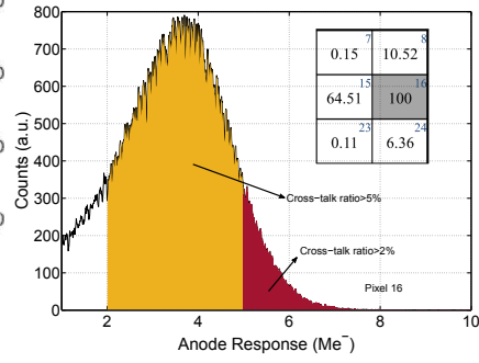
Figure 2.52: Single photon spectra acquired in pixel 16 over a 1 \text{ Me}^- threshold. The table shows the probability (in %) to see a cross-talk signal above 100 \text{ ke}^- threshold in all the neighbouring channels around pixel 16. The pixel numbers are reported in blue in the top-right corner.
