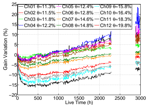
Figure 2.39: Gain variation (in %) versus the illumination period for the third tested MaPMT (FA0025).
