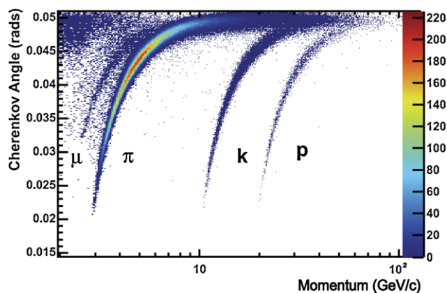
Fig. 14 Reconstructed Cherenkov angle as a function of track momentum in the C_4F_{10} radiator
