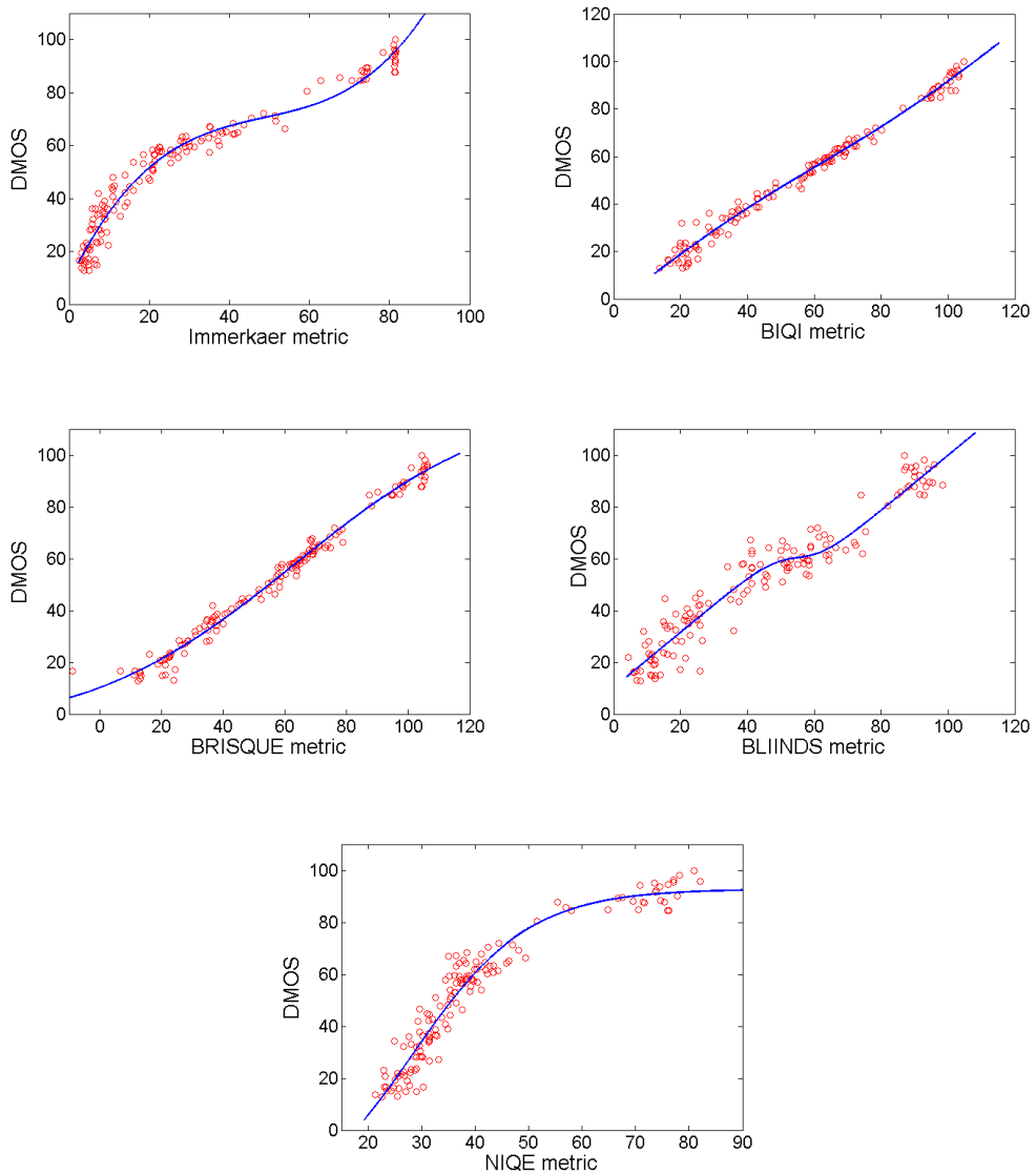
Figure 3.5: Logistic regression for different NR metrics for noise on LIVE data. First row: Immerkaer [51] and BIQL; second row: BRISQUE and BLIINDS; third row: NIQE.
