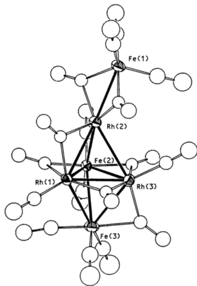
Fig. 1. ORTEP drawing of the [\text{Fe}_3\text{Rh}_3(\text{CO})_{10}(\mu_2\text{-CO})_7]^{3-} tri-anion. Most relevant bond parameters (Å): Rh(1)–Rh(2) 2.771, Rh(1)–Rh(3) 2.682, Rh(2)–Rh(3) 2.869, Rh(1)–Fe(2) 2.714, Rh(1)–Fe(3) 2.802, Rh(2)–Fe(1) 2.575, Rh(2)–Fe(2) 2.819, Rh(3)–Fe(2) 2.673, Rh(3)–Fe(3) 2.716, Fe(2)–Fe(3) 2.770. Average Fe–C, 1.727, Fe–C b , 1.967, Rh–C, 1.821, Rh–C b , 1.996, C–O i , 1.178, C–O b , 1.190. Typical esd's on single distances are: Rh–Rh 0.001, Rh–Fe 0.002, Fe–Fe 0.002, Rh–C 0.01, Fe–C 0.01 and C–O 0.01.
