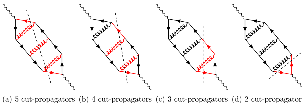
Figure 1. Example of a four-loop massless photon self-energy featuring three internal gluons with different possible choices of cut propagators (in red). According to the number of propagators on cut, the same diagram can represent the integral over the phase space of: (a) a tree-level squared amplitude \gamma \rightarrow qgg\bar{q} , (b) the interference between a one-loop amplitude \gamma \rightarrow qgg\bar{q} with its tree-level, (c) the interference between a two-loop amplitude \gamma \rightarrow qg\bar{q} with its tree-level, (d) the interference between a three-loop amplitude \gamma \rightarrow q\bar{q} with its tree-level.
