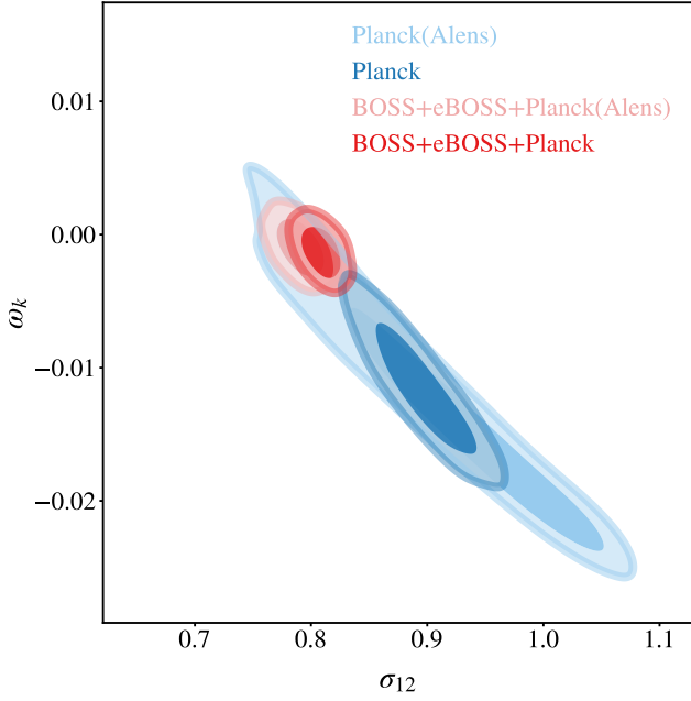
Figure 5. Marginalised posterior contours for \sigma_{12} and \omega_K from Planck and its combination with BOSS+eBOSS in w KCDM. We compare two cases - one with varying A_{\text{lens}} (light blue and pink) and a fiducial one, with A_{\text{lens}} fixed to 1 (dark blue and red).
