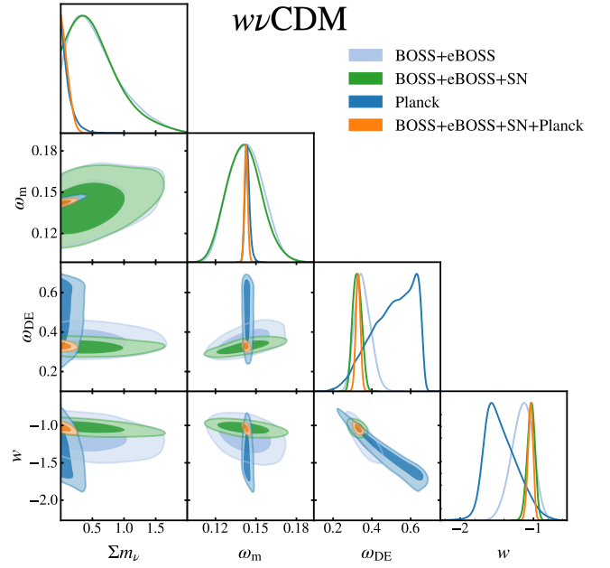
Figure 6. Marginalised posterior contours for dark energy parameters and the neutrino mass sum \Sigma m_\nu in w \nu CDM. Here, we explore varying w together with \Sigma m_\nu . We show constraints from the full-shape clustering analysis of BOSS DR12 galaxies in combination with eBOSS quasars (light blue), their combination with Pantheon SN Ia measurements (green), CMB constraints by Planck (in dark blue) and the combination of all four datasets (in orange).
