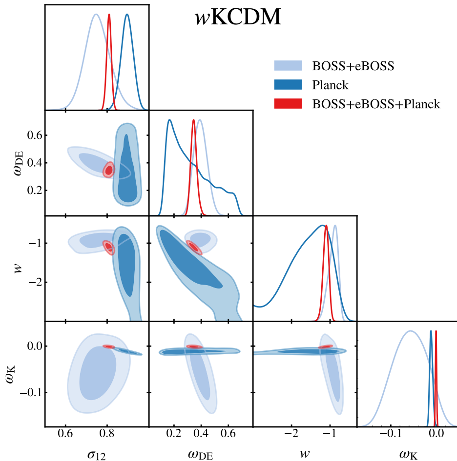
Figure 4. Marginalised posterior contours for dark energy parameters and physical matter and curvature densities in w KCDM, where, in addition to varying w , we also allow for non-zero curvature. The constraints from the full-shape clustering analysis of BOSS DR12 galaxies in combination with eBOSS quasars are shown in light blue, CMB constraints by Planck are displayed in dark blue and the combination of the two sets of probes is shown in red. Note the discrepancy between Planck and BOSS+eBOSS in \sigma_{12} as well as w - \omega_{DE} plane.
