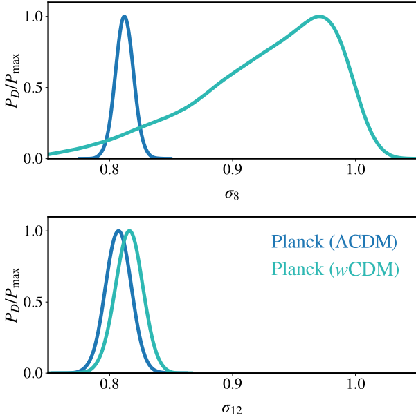
Figure 2. Upper panel: one-dimensional marginalised Planck posteriors for \sigma_8 for \Lambda CDM (blue) and w CDM (green) cosmologies. Lower panel: the corresponding posteriors of \sigma_{12} . The difference between two panels is due to h^{-1} Mpc units used to define the scale at which the linear density field variance is measured for \sigma_8 . As Planck does not constrain H_0 well once w is allowed to freely vary, the resulting posterior, over which the clustering amplitude is effectively averaged, is extremely wide and results in degraded constraint on \sigma_8 . The parameter \sigma_{12} is not affected by this issue, as it is defined on a Mpc scale - the precision of the measurement for Planck is the same in both cosmologies shown.
