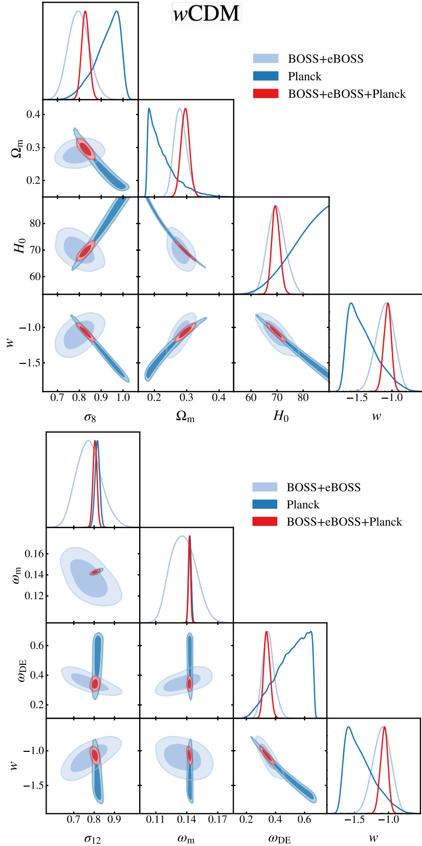
Figure 1. Marginalised posterior contours in the ‘traditional’ and h -independent parameter spaces derived from the full shape of anisotropic clustering measurements of BOSS DR12 galaxies in combination with eBOSS quasars (light blue) and CMB measurements by Planck (dark blue) for a w CDM model. The joint constraints are shown in red. In physical parameter space, Planck is able to constrain the clustering amplitude today \sigma_{12} even in models with free w .
