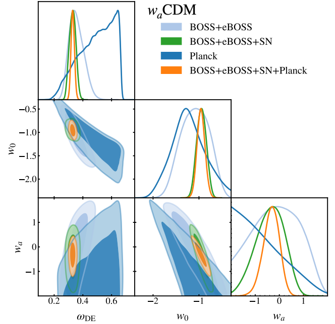
Figure 3. Marginalised posterior contours for dark energy parameters in w_a CDM, where the dark energy equation of state parameter w is allowed to evolve in time, as defined in equation (15). We show constraints from the full-shape clustering analysis of BOSS DR12 galaxies in combination with eBOSS quasars (light blue), their combination with Pantheon SN Ia measurements (green), CMB constraints by Planck (in dark blue), and the combination of all four datasets (in orange).
