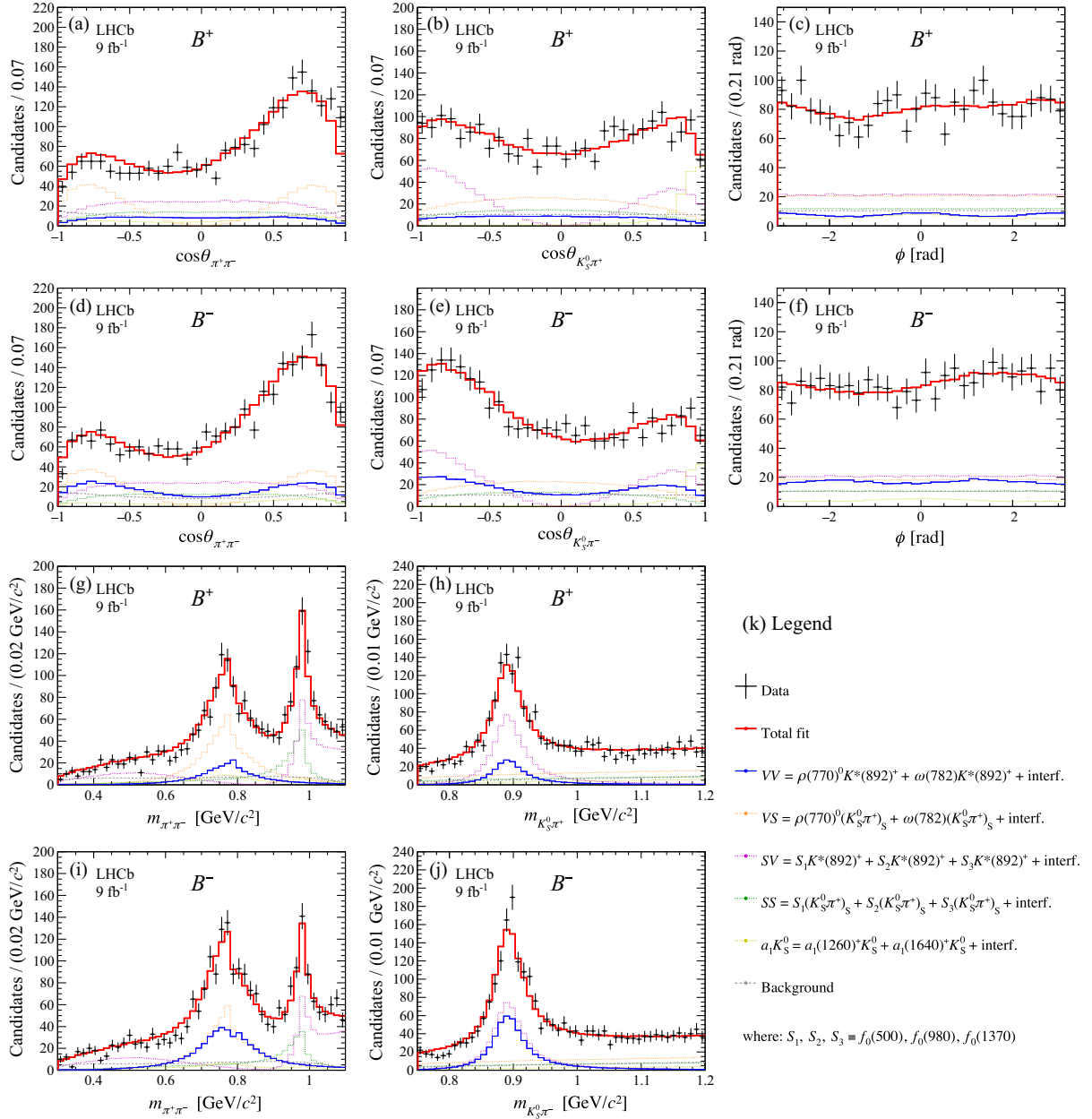
FIG. 2. Projections of the multidimensional amplitude fit onto (a) \cos \theta_{\pi^+\pi^-} , (b) \cos \theta_{K_S^0\pi^+} , (c) \phi , (g) m_{\pi^+\pi^-} , and (h) m_{K_S^0\pi^+} for the B^+ \rightarrow (\pi^+\pi^-)(K_S^0\pi^+) decay. Plots (d)–(f),(i),(j) show the corresponding variables for the B^- \rightarrow (\pi^-\pi^+)(K_S^0\pi^-) decay.
