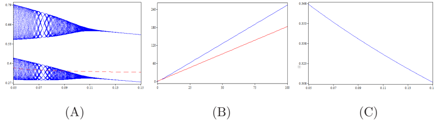
Figure 13: In (A) and (C) we report the bifurcation diagrams of q_{1,t+1} in (3.1) with respect to d \in (0.05, 0.15) with initial conditions q_{1,0} = 0.25 , q_{2,0} = 0.2 for p = 2.5 , \delta = 0.4 , \beta = 3.1 , c = 0.15 , b = 0.4 , \varepsilon = 2.7 , \sigma = 6 , \gamma = -3 , and v = 1.28 in (A), v = 0.5 in (C), respectively. In (B) we show the time series of cumulative emissions CE_T for T \in [0, 100] corresponding to (A) with d = 0.1 , with initial conditions u_{1,0} + u_{2,0} = 1.215 , connected with q_{1,0} = 0.25 and q_{2,0} = 0.2 , for the blue points, and 2\varepsilon q_1^* = 2 * 2.7 * 0.336 = 1.814 for the red points.
