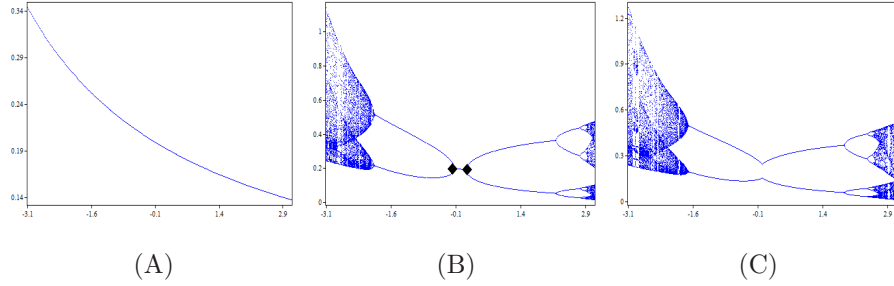
Figure 7: The bifurcation diagram of q_{1,t+1} in (3.1) for \gamma \in (-3.1, 3.1) and initial conditions q_{1,0} = 0.25 , q_{2,0} = 0.2 , for p = 2.5 , \delta = 0.4 , v = 2.2 , \beta = 3.1 , c = 0.15 , b = 0.4 , d = 0.1 , \varepsilon = 2.7 , and \sigma = 2 in (A), \sigma = 5.8 in (B), \sigma = 6 in (C).
