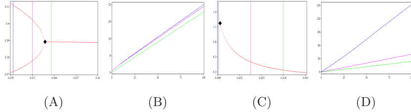
Figure 8: In (A) and (C) we report the bifurcation diagrams of U_{t+1} with respect to d for the same parameter values used in Figs. 4 (C) and 6 (B), respectively. In (B) and (D) we show the time series of cumulative emissions CE_T for T \in [0, 100] corresponding to the values of d marked with different colors in (A) and (C), respectively. The initial conditions in (B) are U_0 = \varepsilon(q_{1,0} + q_{2,0}) = 2.7 * 0.45 = 1.215 , connected with q_{1,0} = 0.25 and q_{2,0} = 0.2 , for the blue and the red time series, and 2\varepsilon q_1^* = 2 * 2.7 * 0.052 = 0.281 for the green time series, while in (D) the initial conditions are U_0 = 2.7 * 0.45 = 1.215 , connected with q_{1,0} = 0.25 and q_{2,0} = 0.2 , for the blue time series, 2\varepsilon q_1^* = 2 * 2.7 * 0.074 = 0.399 for the red time series, and 2\varepsilon q_1^* = 2 * 2.7 * 0.044 = 0.238 for the green time series.
