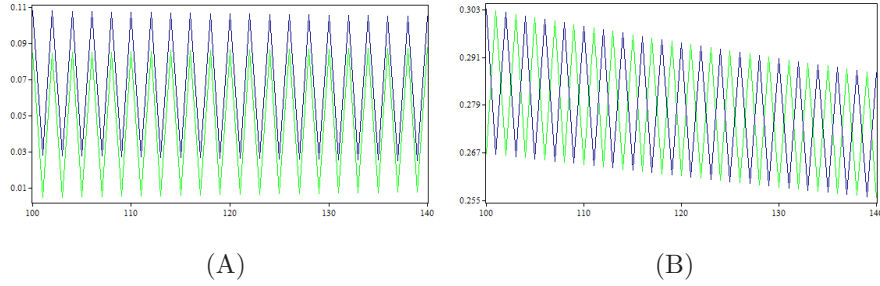
Figure 9: In (A) and (B) we show the time series of q_{1,t} in dark blue and of q_{2,t} in green for t \in [101, 140] , corresponding to the values of d marked in blue in Fig. 8 (A) and (C), respectively.
