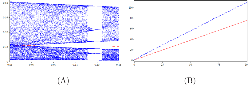
Figure 10: In (A) the bifurcation diagram of q_{1,t+1} in (3.1) with respect to d \in (0.05, 0.15) with initial conditions q_{1,0} = 0.1 , q_{2,0} = 0.5 , for p = 2.5 , \delta = 0.4 , v = 2.2 , \beta = 3.1 , c = 0.15 , b = 0.4 , \varepsilon = 2.7 , \sigma = 6 and \gamma = 3 . In (B) we show the time series of cumulative emissions CE_T for T \in [0, 100] corresponding to d = 0.1 , with initial condition u_{1,0} + u_{2,0} = 1.62 , connected with q_{1,0} = 0.1 and q_{2,0} = 0.5 , for the blue points and 2\varepsilon q_1^* = 2 * 2.7 * 0.139 = 0.751 for the red points.
