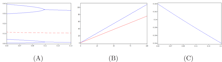
Figure 11: In (A) and (C) we report the bifurcation diagrams of q_{1,t+1} in (3.1) with respect to d \in (0.05, 0.15) with initial conditions q_{1,0} = 0.1 , q_{2,0} = 0.5 , for p = 2.5 , \delta = 0.4 , \beta = 3.1 , c = 0.15 , b = 0.4 , \varepsilon = 2.7 , \sigma = 6 , \gamma = 3 , and v = 1.35 in (A), v = 0.5 in (C), respectively. In (B) we show the time series of cumulative emissions CE_T for T \in [0, 100] corresponding to (A) with d = 0.1 , with initial conditions u_{1,0} + u_{2,0} = 1.62 , connected with q_{1,0} = 0.1 and q_{2,0} = 0.5 , for the blue points and 2\varepsilon q_1^* = 2 * 2.7 * 0.139 = 0.751 for the red points.
