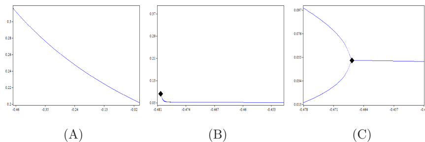
Figure 4: The bifurcation diagram of q_{1,t+1} in (3.1) with respect to d and initial conditions q_{1,0} = 0.25 , q_{2,0} = 0.2 , for \delta = 0.4 , \nu = 2.2 , \beta = 3.1 , c = 0.15 , b = 0.4 , \varepsilon = 2.7 , \gamma = 3 , and p = 3 , \sigma = 1.478 in (A), p = 1.4 , \sigma = 1.478 in (B), p = 1.4 , \sigma = 3 in (C).
