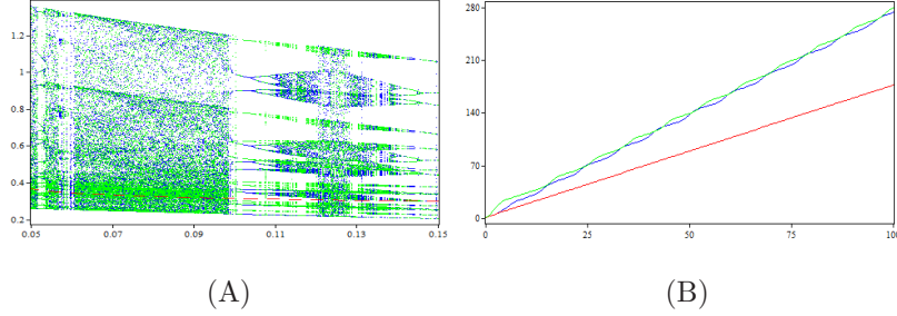
Figure 12: In (A) the bifurcation diagram of q_{1,t+1} in (3.1) with respect to d \in (0.05, 0.15) with initial conditions q_{1,0} = 0.25 , q_{2,0} = 0.2 for the blue points and q_{1,0} = 0.1 , q_{2,0} = 0.5 for the green points, for p = 2.5 , \delta = 0.4 , v = 2.2 , \beta = 3.1 , c = 0.15 , b = 0.4 , \varepsilon = 2.7 , \sigma = 6 and \gamma = -3 . In (B) we show the time series of cumulative emissions CE_T for T \in [0, 100] corresponding to d = 0.1185 , with initial condition u_{1,0} + u_{2,0} = 1.215 , connected with q_{1,0} = 0.25 and q_{2,0} = 0.2 , for the blue points, u_{1,0} + u_{2,0} = 1.62 , connected with q_{1,0} = 0.1 and q_{2,0} = 0.5 , for the green points, and 2\varepsilon q_1^* = 2 * 2.7 * 0.325 = 1.757 for the red points.
