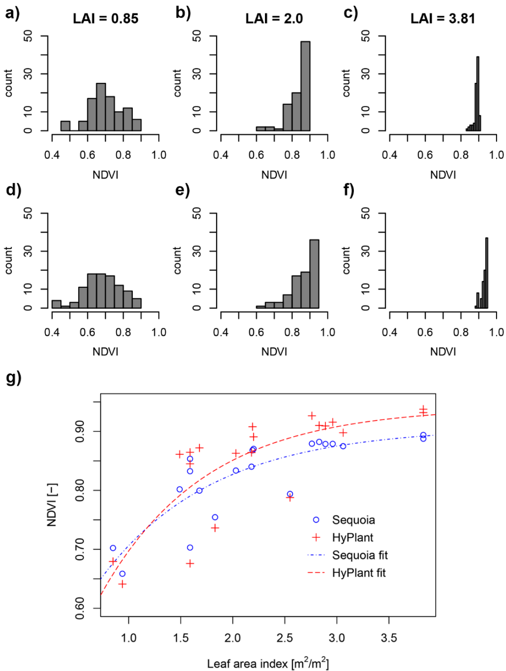
Figure 11. Histograms of Sequoia (a–c) and HyPlant (d–f) NDVI values for three 10 × 10 m ESUs of varying LAI. (g) NDVI values averaged over ESU extents and the corresponding LAI value measured in the field. Non-linear model fits are provided for illustrative purposes.
