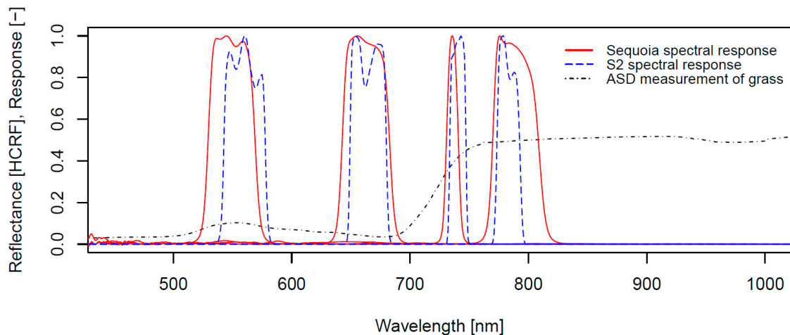
Figure 3. Relative spectral responses of the four Parrot Sequoia cameras as well as the most closely corresponding Sentinel 2A bands (bands 3, 4, 6 and 7), overlaid on a measured grass reflectance spectrum.
