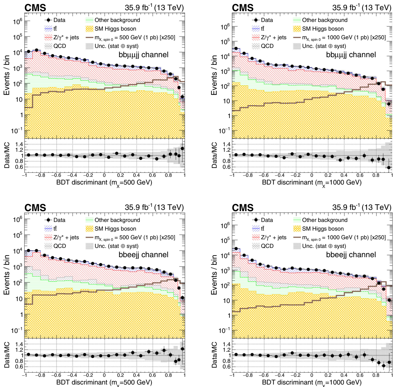
FIG. 1. Comparison of the BDT discriminant for m_X = 500 and 1000 GeV after the final selection in the muon (upper row) and electron (lower row) final states of the bb\ell\ell jj channel. The signals of a RS1 radion with mass of 500 (left panels) and 1000 GeV (right panels) are normalized to a cross section of 1 pb for the pp \rightarrow X \rightarrow hh process. The shaded area represents the combined statistical and systematic uncertainties in the background estimate.
