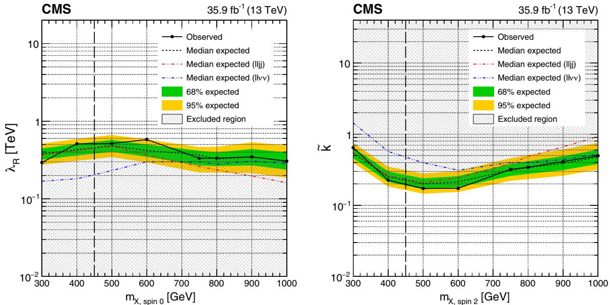
FIG. 5. The expected and observed exclusion limits at 95% CL on the RS1 radion with kL = 35 (RS1 KK graviton) hypothesis in the \lambda_R ( \tilde{k} ) versus mass plane for the individual bb\ell\ell jj (red) and bb\ell\ell\nu\nu (blue) channels and their combination (black). The dark green and light yellow expected limit uncertainty bands represent the 68% and 95% confidence intervals. Solid lines represent the observed limits and dashed lines represent the expected limits. The shaded region is excluded by the current limits. The vertical black dashed line indicates the resonance mass of 450 GeV, a mass point where the BDT used in the bb\ell\ell\nu\nu analysis is switched from the one trained for low-mass resonance to the one trained for high-mass resonance.
