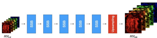
Fig. 1 The overall network architecture of the proposed ESSPN network
