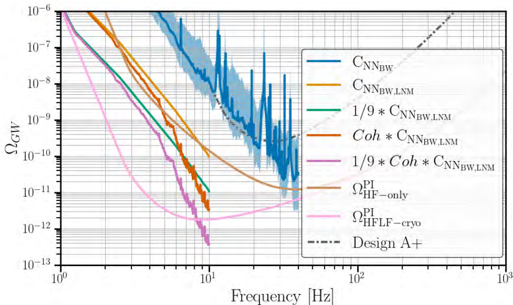
Figure 34: The projected impact from correlated NN from body-waves C_{NN_{BW}} , as calculated in Section III of [141], is shown in blue. The blue line represents the median value, and the associated surface is delimited by the 10% and 90% percentiles. Also curves with more optimistic assumptions (see the text) are shown. Based on Fig. 16 of [141].
