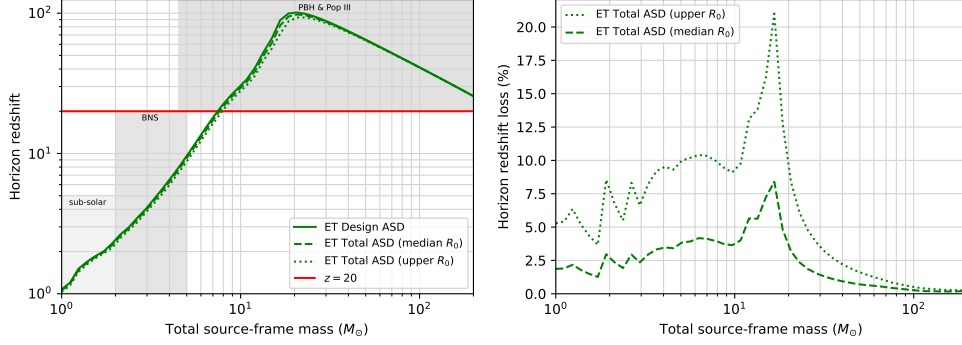
Figure 69: The loss in the ET detection horizon, as estimated in [516], due to the confusion of instrumental noise and compact binary inspirals. Dashed lines show the effect of the median local merger rate and dotted lines represent the upper merger rate. A higher merger rate introduces a stronger confusion noise and hence the higher horizon redshift loss. This effect can be mitigated by the ET null stream available in the \Delta configuration.
