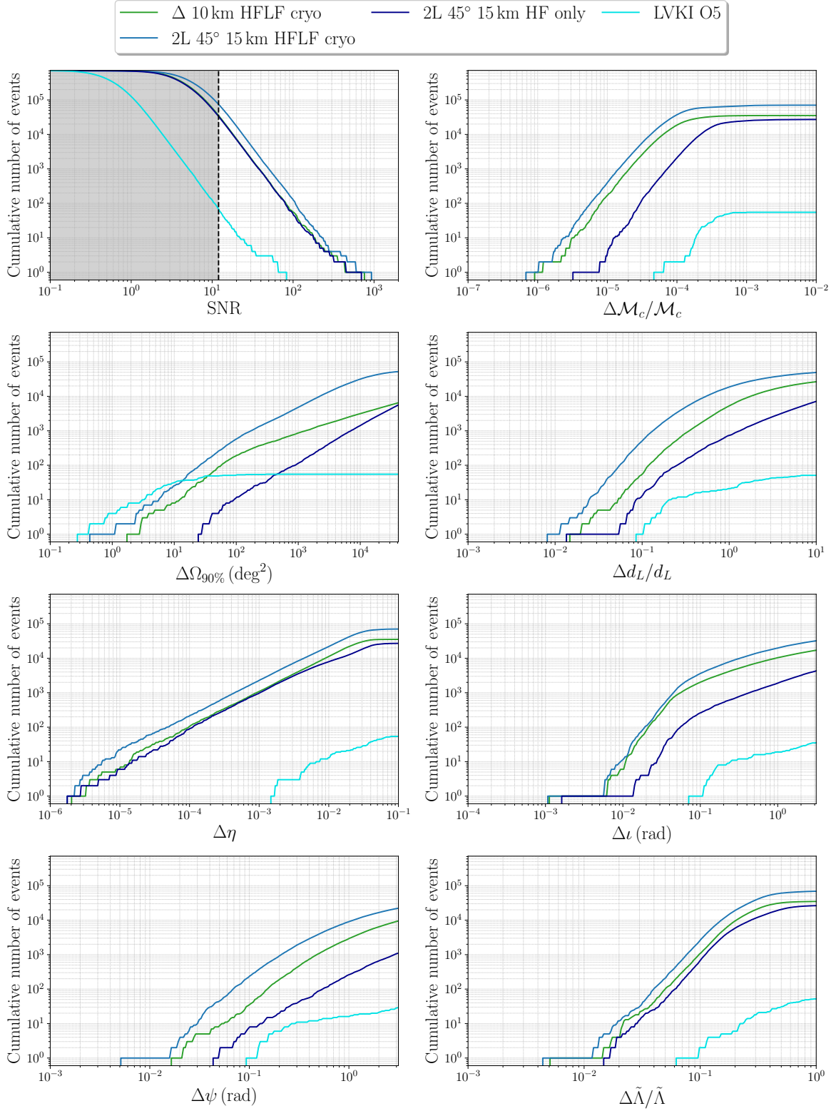
Figure 15: Comparison of SNR and parameter estimation error for the 2L with 15 km arms at 45^\circ , with the two different ASDs. For comparison, we also show the 10 km triangle at full sensitivity, and the forecast for LVKI O5.
