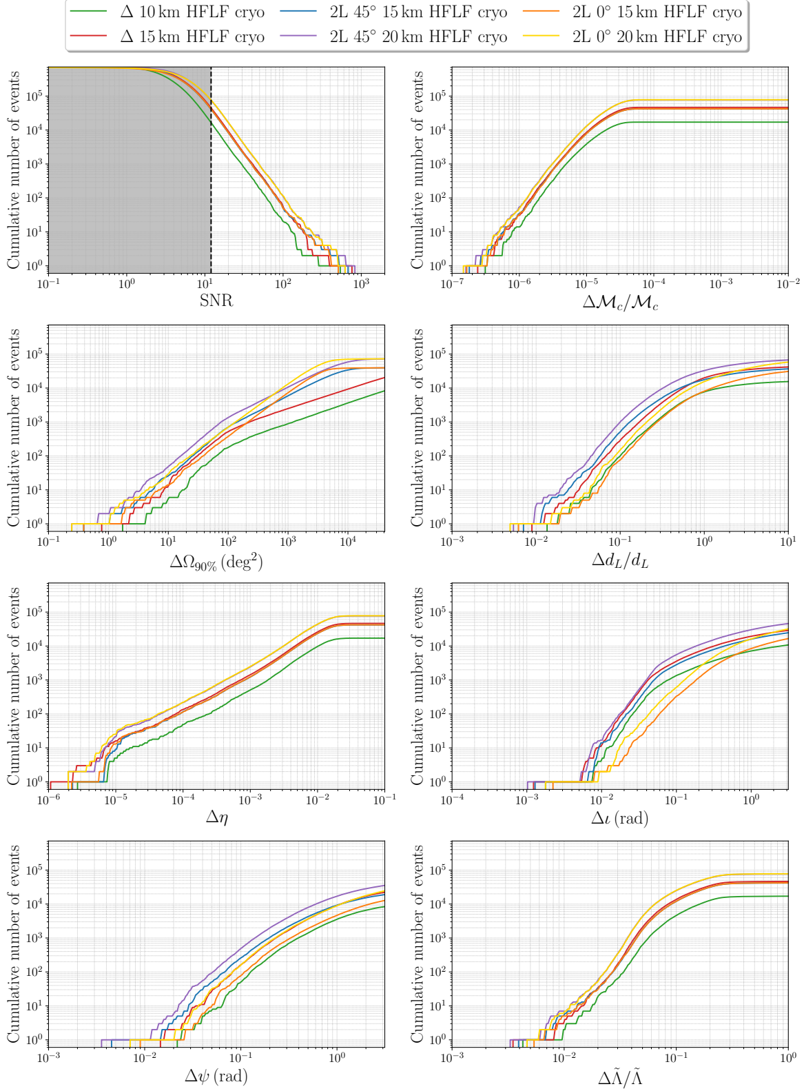
Figure 17: As in Fig. 11, for a gaussian mass distribution of the two component neutron stars.
