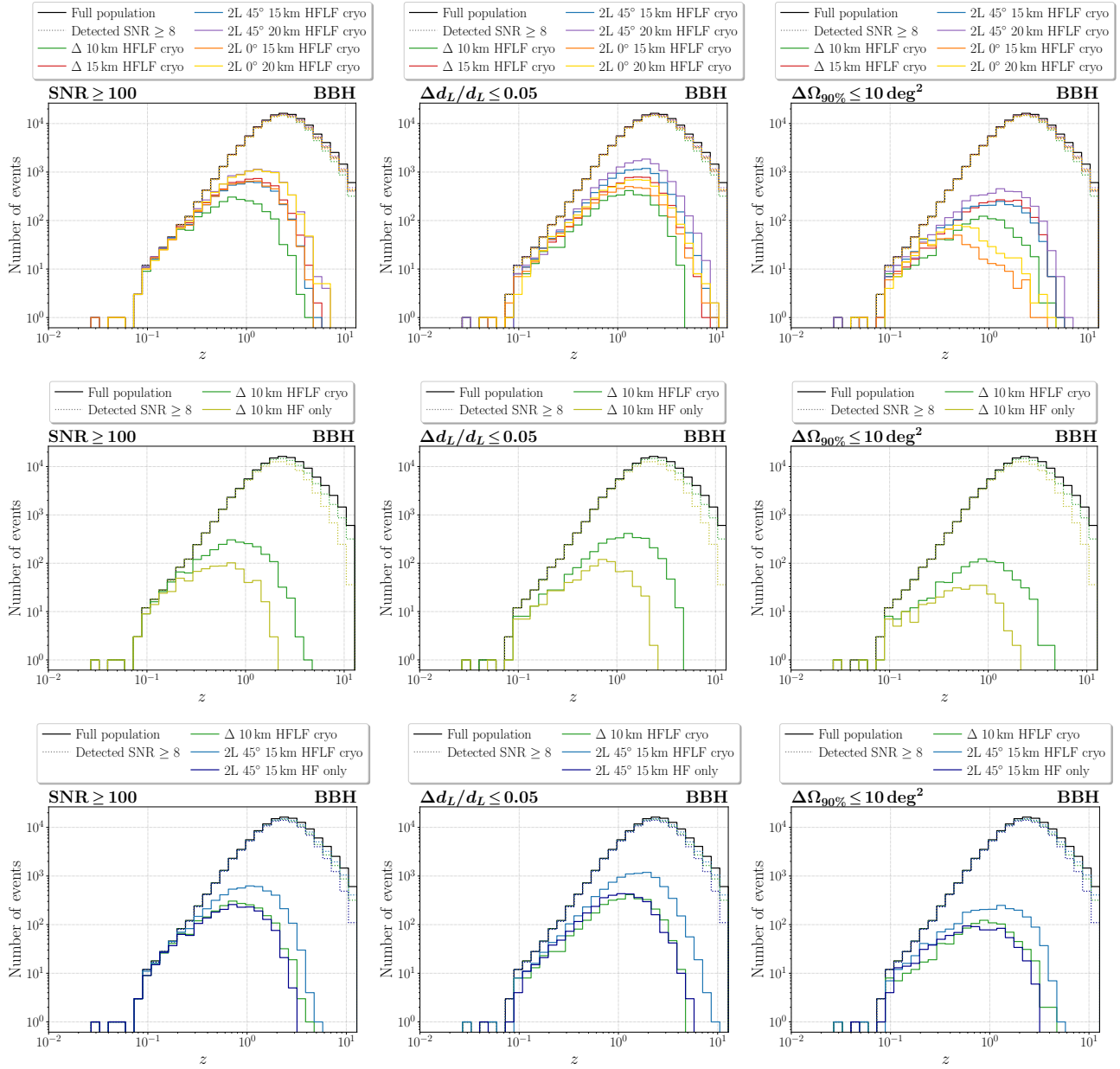
Figure 10: Redshift distribution of BBHs detected with \text{SNR} \geq 100 (left column), or with relative error on the luminosity distance \Delta d_L/d_L \leq 0.05 (central column), or with sky location \Delta\Omega \leq 10 \text{ deg}^2 (right column) for various detector geometries and sensitivity curves. The upper row shows the results for the six considered geometries, all with their best sensitivity, the central row for the 10 km triangle with the two considered ASDs, and the bottom row for the 2L with 15 km arms at 45^\circ and the two considered ASDs (together with the 10 km triangle with the full ASD). In each panel we also show, for reference, the redshift distribution of the BBH population used (black solid line), and of the events detected in the various configurations with \text{SNR} \geq 8 (dotted lines).
