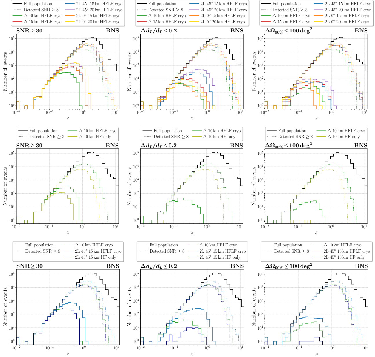
Figure 16: Redshift distribution of BNS detected with \text{SNR} \geq 30 (left column), or relative error on the luminosity distance \Delta d_L/d_L \leq 0.2 (central column), or with sky location \Delta\Omega \leq 100 \text{ deg}^2 (right column) for various detector configurations and sensitivity curves. The upper row shows the results for the six considered geometries, all with their best sensitivity, the central row for the 10 km triangle with the two considered ASDs, and the bottom row for the 2L with 15 km arms at 45^\circ and the two considered ASDs. In each panel, we also show, for reference, the redshift distribution of the BNS population used (black solid line) and the events detected in the various configurations with \text{SNR} \geq 8 (dotted lines).
