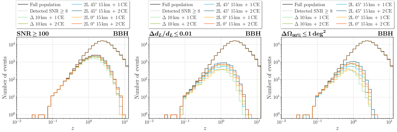
Figure 20: Redshift distribution of detected BBHs with \text{SNR} \geq 100 (left column), or relative error on the luminosity distance \Delta d_L/d_L \leq 0.01 (central column), or sky location \Delta\Omega \leq 1 \text{ deg}^2 (right column), for the six 3G the detector networks considered. In each panel, we also show, for reference, the redshift distribution of the BBH population used (black solid line), and of the events detected in the various configurations with \text{SNR} \geq 8 (dotted lines, graphically almost indistinguishable from the full population on this scale).
