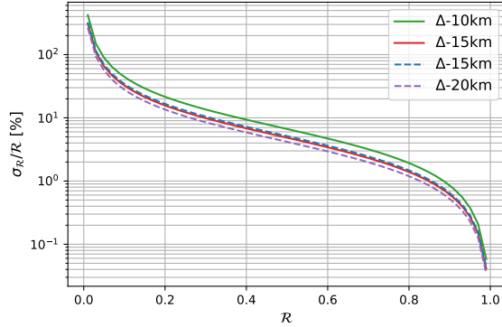
Figure 38: Fractional percentage errors on the ECO reflectivity \mathcal{R} for a GW150914-like event placed at d_L = 1 Gpc with final mass M_f = 70M_\odot and final spin \chi_f = 0.68 . The detector is taken in the cryogenic HFLF configuration and errors are averaged over the sky position and the inclination angle. There are no significant deviations in the figure for the HF-only configuration. The Fisher-matrix parameters are \{M_f, \chi_f, \mathcal{R}, \phi(\mathcal{R}), \epsilon\} , where \mathcal{R} is generically a complex number, and the amplitude and phases \{\mathcal{A}_{lmn}, \phi_{lmn}\} of the excited modes.
