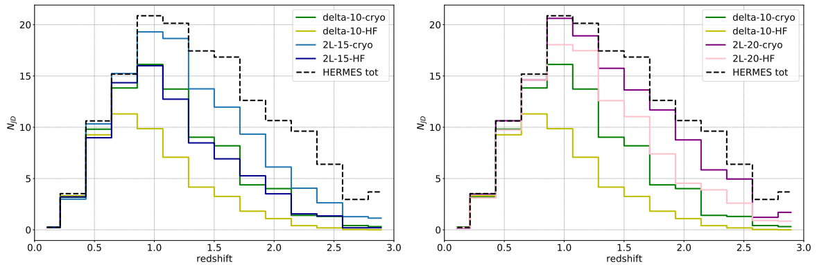
Figure 24: Histogram of the joint detection of ET and HERMES observing in survey mode during one year. The plot shows the comparison among ET full sensitivity and ET HF for \Delta 10 km and 2L15km (left plot), and 2L20km (right plot). The dashed line show the prompt emission of short \gamma -ray bursts expected to be detected by HERMES during one year of observations.
