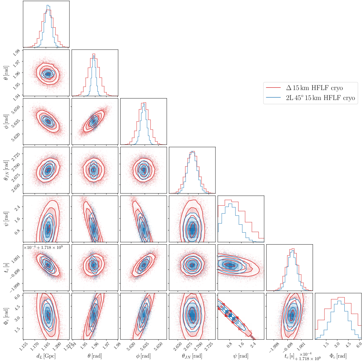
Figure 73: As in Fig. 72 for a BBH event with heavier masses and greater distance (“event 2”, see the text).
