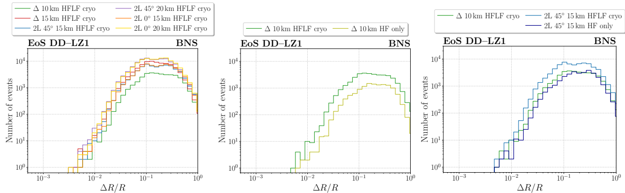
Figure 41: Distribution of the relative errors on the NS radius attainable from the adimensional tidal deformability combination \tilde{\Lambda} , as measured by different detector configurations and sensitivity curves. In particular, the left panel shows the results for the six geometries considered, all with their best sensitivity, the central panel for the 10 km triangle with the two different ASDs, and the right panel for the 2L with 15 km arms at 45^\circ and the two ASDs considered.
