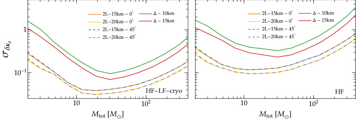
Figure 39: 1\text{-}\sigma uncertainty on the parameter controlling deviations on the symmetric combination of the spin-induced ECO quadrupole moment, \kappa_s = 1 + \delta\kappa_s , with \kappa_s = 1 corresponding to binaries with Kerr BHs. We assume the Kerr case ( \delta\kappa_s = 0 ) and optimally-oriented sources with mass ratio q = 2 , non-precessing spins \chi_1 = 0.9 , \chi_2 = 0.7 at a luminosity distance of d_L = 100 Mpc. The optimal orientation depends on the detector location and configuration. The Fisher-matrix parameters are \{\mathcal{M}_c, \eta, d_L, \theta, \phi, \iota, \psi, t_c, \Phi_c, \chi_{1,z}, \chi_{2,z}, \delta\kappa_s\}
