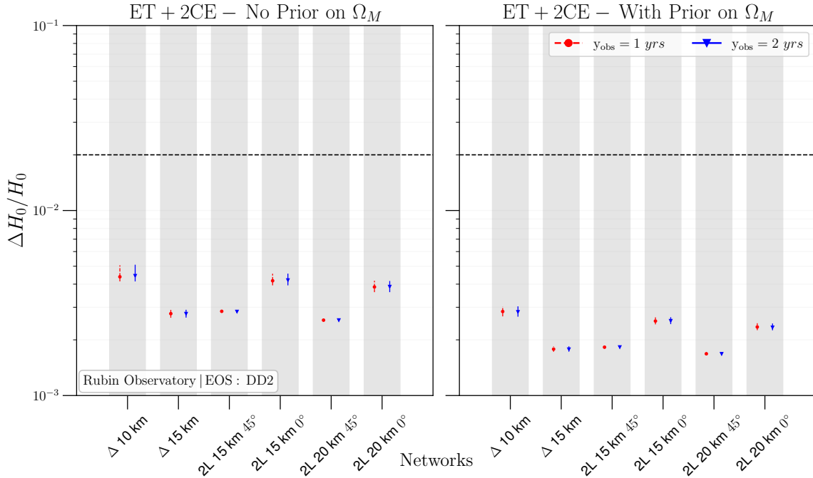
Figure 62: Same as Fig. 61 except the results are obtained for the NSBH population instead of the BBH population. Moreover, the results were obtained by combining measurement accuracies from systems that produce kilonovae in addition to those that identify a unique host within the localization error box.
