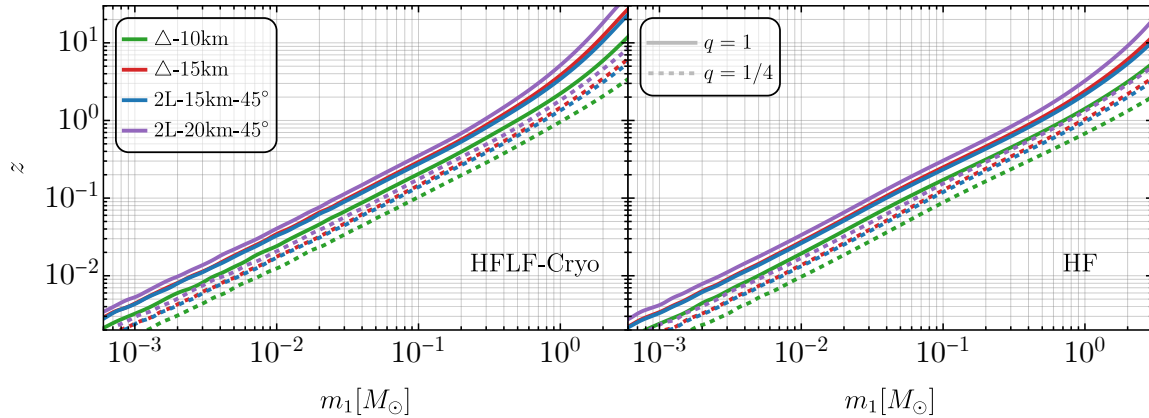
Figure 49: Detection horizons for non-spinning PBH binaries assuming a mass ratio q = 1 or q = 1/4 , for the various detector configurations considered. This plot extends Fig. 3 in the sub-solar mass range, of interest for PBHs.
