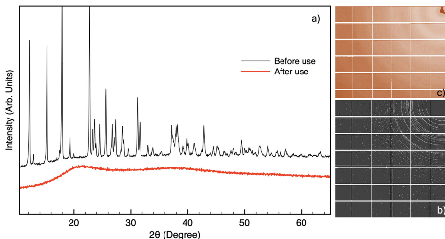
Fig. 5 (a) XRD patterns of the malate material before (black line) and after (red line) the photothermo-catalytic tests. Before the functional test, all the peaks in the XRD pattern can be attributed to the newly detected phase \text{MH}_2(\text{C}_4\text{H}_4\text{O}_5)_2 \cdot 4\text{H}_2\text{O} , with M representing the metals. 2D images of XRD patterns of the malate phase (b) before and (c) after photocatalytic tests collected under synchrotron radiation are also shown.
