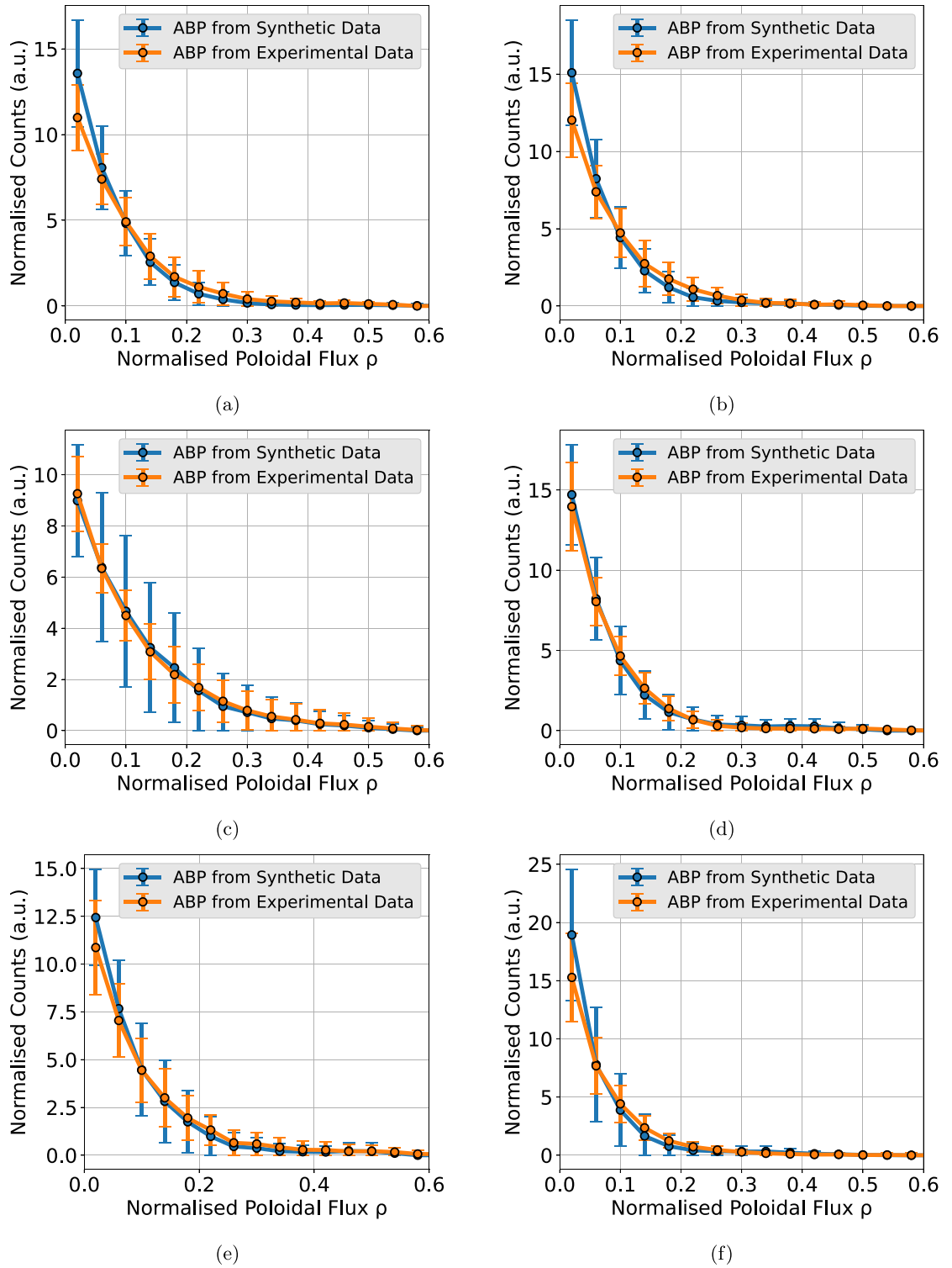
Figure 12. Comparisons between experimental (orange) and synthetic (blue) normalized alpha emissivity profiles as a function of the normalized poloidal flux coordinate \rho , for all the remaining analysed discharges. (a): 95 672-A25; (b): 95 673-A26; (c): 95 679-V36; (d): 95 680-V07; (e): 95 683-V07; (f): 95 684-A24.
