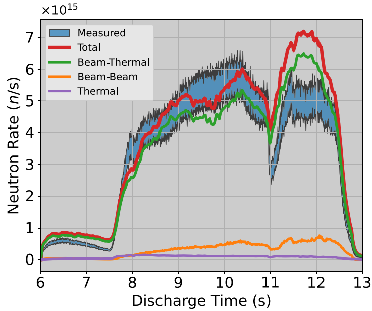
Figure 8. Comparison between TRANSP-simulated and experimentally measured total neutron rate for discharge 95 671 at JET. Blue: experimental measurement bounds. Red: TRANSP-predicted total neutron rate. Green: D beam–thermal D contribution. Orange: beam–beam contribution. Purple: thermal–thermal contribution. Simulation ID: ‘A25’. Experimental data from fission chambers at JET. Time offset of 40 s.
