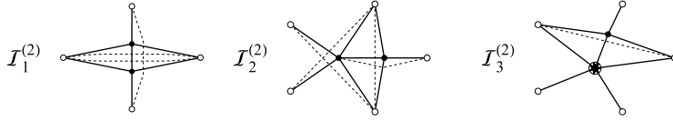
Figure 3. Two loop five-point parity even ( \mathcal{I}_1^{(2)} and \mathcal{I}_2^{(2)} ) and parity odd ( \mathcal{I}_3^{(2)} ) amplitude graphs. The starred vertex v indicates a factor i_{\epsilon_{12345v}} .
