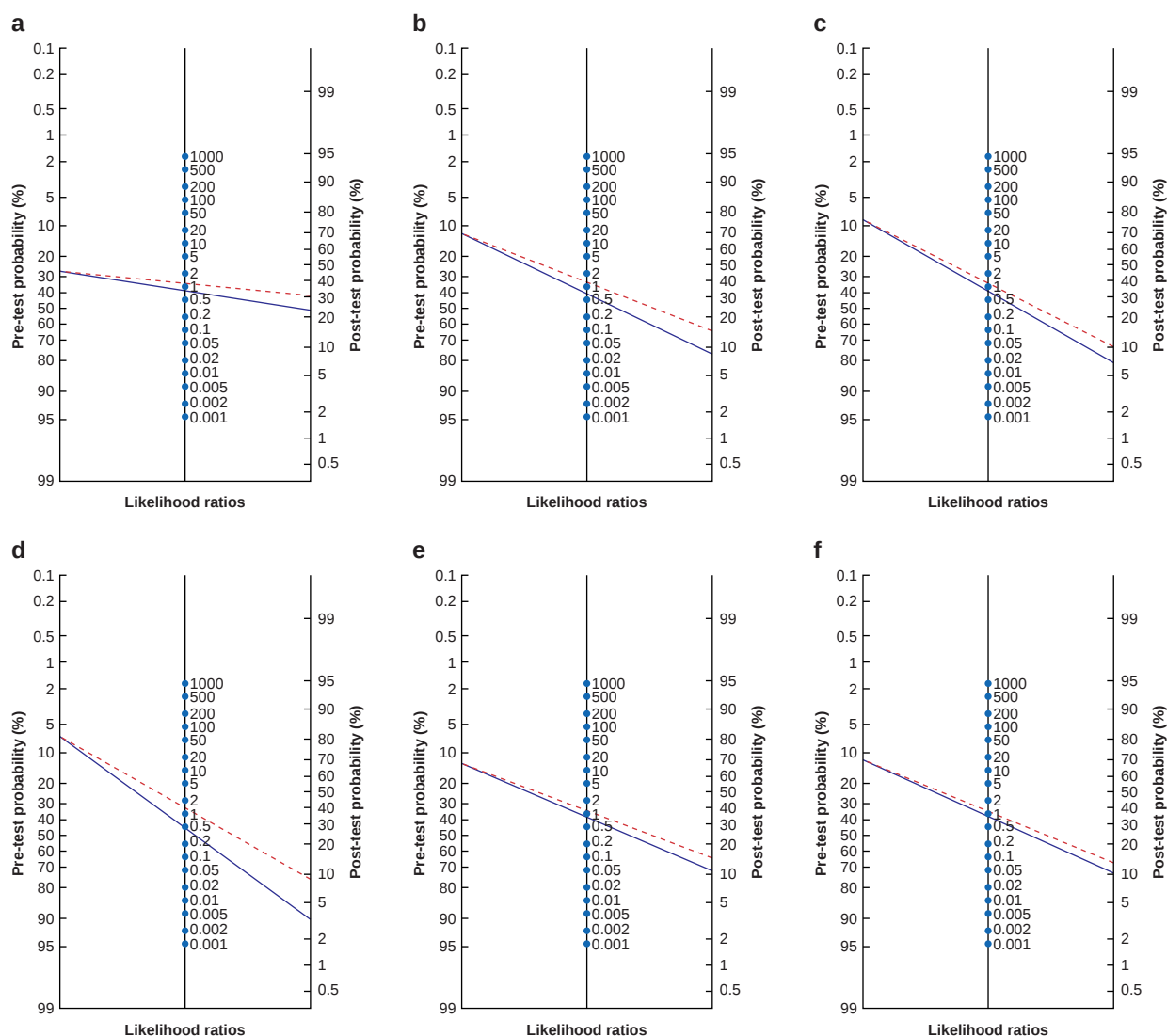
Fig. 2 Nomograms of pre- and post-test probabilities and likelihood ratios of an NRS greater than or equal to seven
