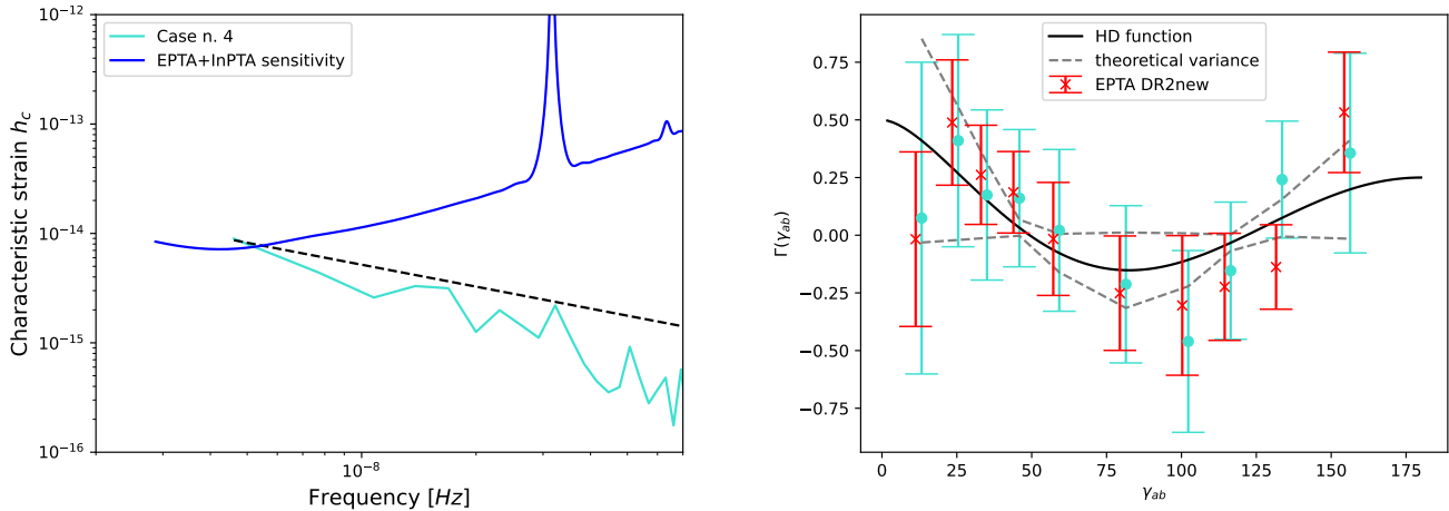
Fig. 11: Case4 analysis. The left panel shows the characteristic strain spectrum compared to the f^{-2/3} trend (dashed black line). The sensitivity curve is the one presented in Collaboration et al. (2023). Right panel: comparison between the recovered angular correlation in the residuals for this specific realisation (light blue points) and the results for the EPTA DR2new dataset (red). The expected variance of the optimal correlation estimator, for the EPTA 25 best pulsars array, is derived from prescriptions in Allen & Romano (2023).
