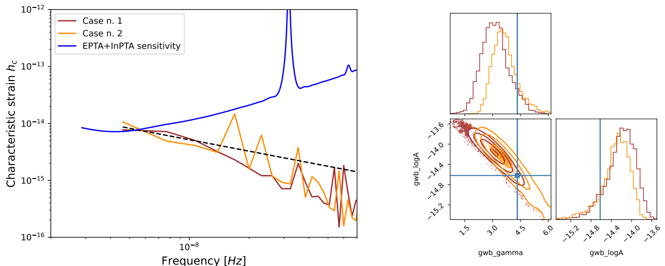
Fig. 9: Comparison between the two realisations denoted as Case1 and Case2 . In the left panel we compare the characteristic spectra with the the f^{-2/3} trend, represented by the dashed black line. The sensitivity curve is the one presented in Collaboration et al. (2023). Right panel: corner plot of the GWB parameter posteriors for Case1 (brown posterior) and 2 (orange posterior). The simulated GWB amplitude is 2.4 \times 10^{-15} .
