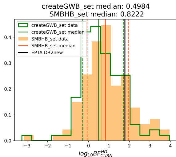
Fig. 7: Histograms of the \log_{10}\text{BF}_{\text{CURN}}^{\text{HD}} obtained from the reweighting analysis on the createGWB_set (green) and SMBHB_set (orange). The solid vertical lines show the medians of the distributions, while the dashed ones refer to the 16th and 84th percentiles. The black vertical line corresponds to the latest EPTA estimate for DR2new: \text{BF}_{\text{CURN}}^{\text{HD}} \sim 60 .
