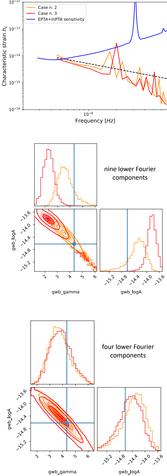
Fig. 10: Notable realisations Case2 (orange) and Case3 (red). Top panel: GWB spectra. The dashed black line represents the f^{-2/3} trend. The sensitivity curve is the one presented in Collaboration et al. (2023). The central and bottom panels show corner plots of the GWB parameter posteriors inferred from the analysis using nine (central panel) and four (bottom panel) frequency bins for the GWB recovery.
