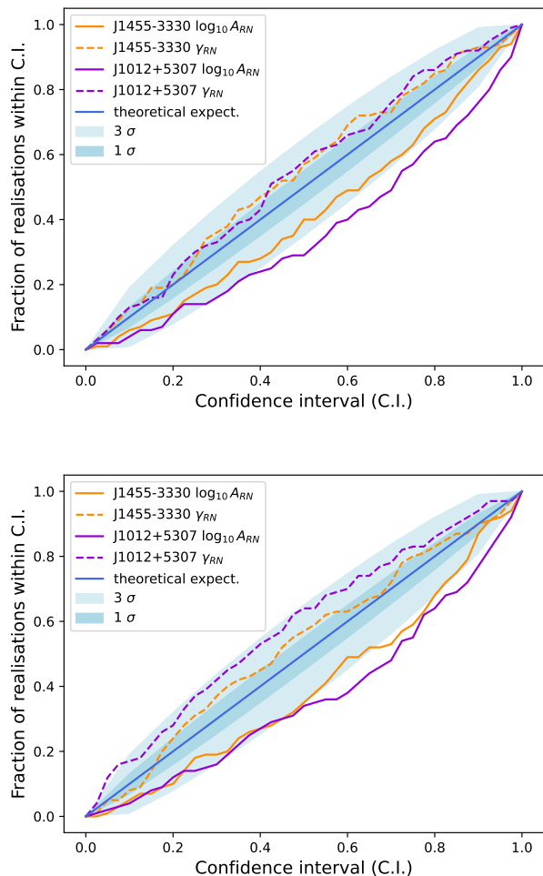
Fig. A.1: P–P plots for the recovery of pulsars J1455-3330 and J1012+5307 RN parameters from the MCMC inference runs performed on the createGWB (top panel) and SMBHB_set (bottom). Dashed lines are for the power-law slope, while the solid lines refer to the RN amplitude.
