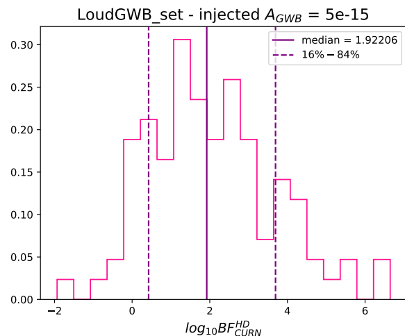
Fig. 3: \log_{10}BF distribution of HD vs CURN for the 100 realisations of the LoudGWB_set . The vertical lines show the median (solid) and the 16th and 84th percentile (dashed) of the distribution.
