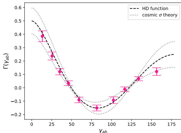
Fig. 4: HD correlation recovery for the LoudGWB_set . Each data point corresponds to the average of the optimal correlation estimators in that bin over all realisations. The expected cosmic variance is derived in Allen (2023).
