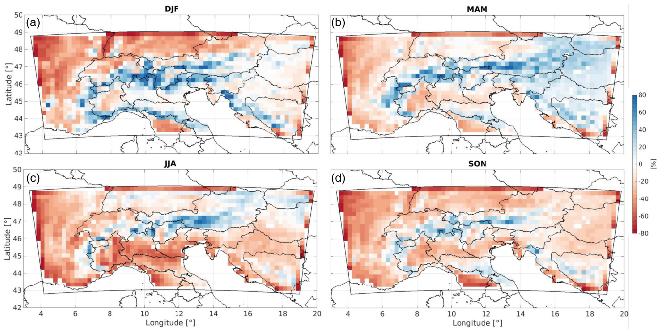
FIGURE 5 Difference (in percentage) of mean seasonal precipitation between WRF-historical and ERA5 (1979–2008). WRF data has been interpolated onto the ERA5 grid
