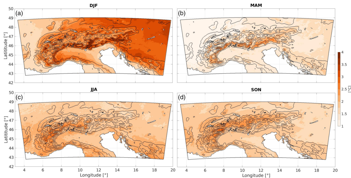
FIGURE 7 Map of the difference between future (2039–2068) and historical WRF simulation (1979–2008) in seasonal mean 2 m temperature: DJF (a), MAM (b), JJA (c) and SON (d). Isolines represent the elevation every 500 m
