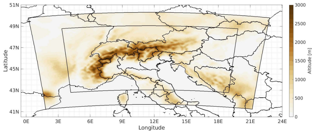
FIGURE 1 Two grafted domains that represent the GAR used in this model study. The topography of the inner domain (4 km resolution) and of the external domain (12 km) are represented
