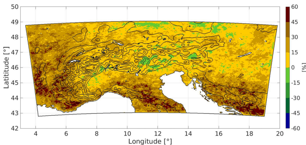
FIGURE 15 Relative change to the climatological average maximum number of consecutive dry days per year (1979–2008, 2039–2068), CDD index
