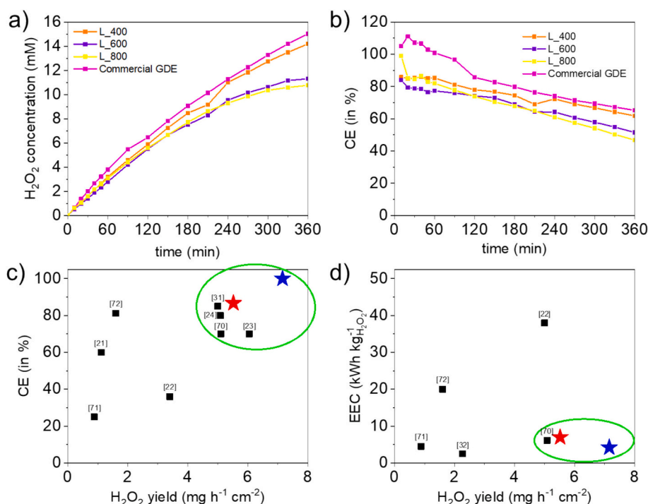
Fig. 7. a) Time course of (a) H 2 O 2 concentration and (b) current efficiency for the galvanostatic electrolysis of 150 mL of 0.05 M Na 2 SO 4 medium at pH 5.9 and 10 mA cm -2 , using metal-free non-activated carbons obtained from pyrolysis at 400, 600 and 800 °C, along with a commercial GDE. The electrocatalyst loading in the GDEs was 0.5 mg cm -2 . In addition, comparison of the performance of L 400 and commercial GDE (red and blue star, respectively) with respect to that of biomass-derived GDEs reported in the literature [21–24,31,32,70–72] in terms of: c) current efficiency vs H 2 O 2 yield and b) electrical energy consumption vs H 2 O 2 yield. The green circle on top right in plot c and on bottom right in plot d highlights the desired performance. (For interpretation of the references to color in this figure legend, the reader is referred to the web version of this article.)
