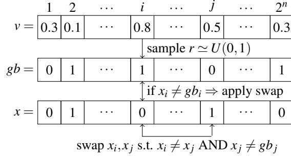
Figure 1: Example of application of swap-based position update.
