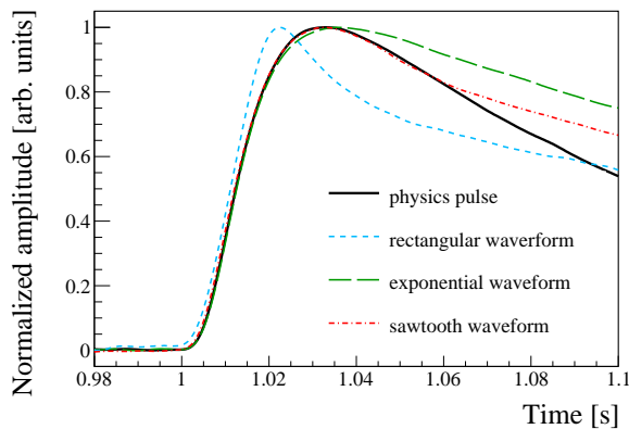
FIG. 1. Overlay of the rising edge and initial part of the decay for heater pulses excited by rectangular (blue, en-dashed), exponential (green, em-dashed) and sawtooth (red, dot-dashed) waveforms and a particle pulse (black). Particle pulses have a similar shape, despite the different origin and entity of the energy deposition; quantitatively, the width of the distribution of rise and decay time is close to 3%.
