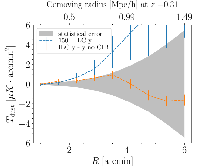
FIG. 25. Same as Fig. 21 but for LOWZ instead of CMASS. Here again, the dust contribution to the measured tSZ+dust profiles is non-negligible, as expected.
