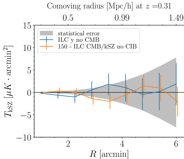
FIG. 24. Same kSZ foreground null tests as Fig. 21 but for LOWZ instead of CMASS.
