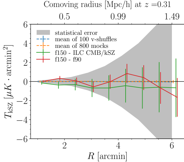
FIG. 23. Same kSZ pipeline null tests as Fig. 20 but for LOWZ instead of CMASS.
