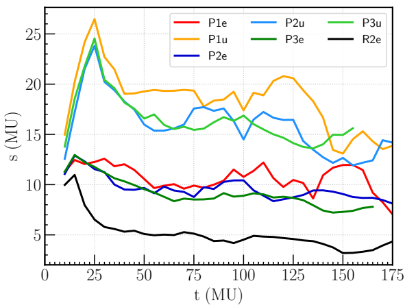
Figure 5. Time evolution of the hardening rates (Eq. 6) for the different runs presented in the paper.
