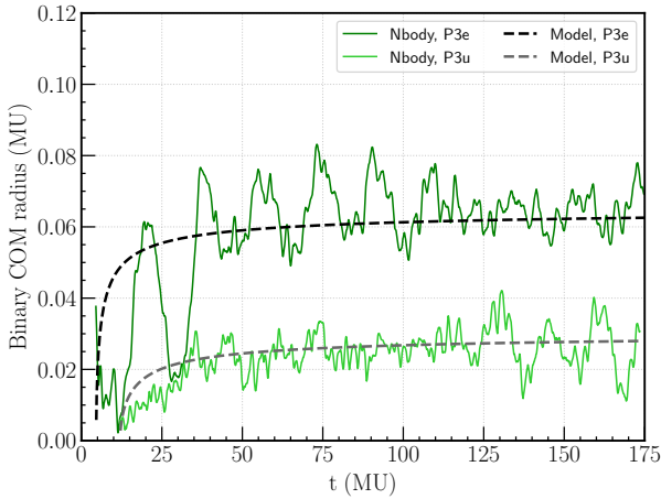
Figure 8. Time evolution of the binary CoM displacement from the centre of the system, R_b , as obtained from the simulations (solid lines) and from our theoretical modelling (Eq. 11). For model P3e we solved Eq. (11) assuming \rho = 0.8 , \sigma = 0.7 , a_0 = 0.05 , s = 10 and we initialize R_b = 0 at t = 7.5 ; for model P3u we set \rho = 2 , \sigma = 0.75 , a_0 = 0.01 , s = 15 and we initialize R_b = 0 at t = 12 . These are characteristic values we extracted from the simulation. The most uncertainty is associated to the choice of a_0 , as better detailed in the text and in footnote 9.
