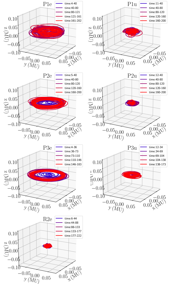
Figure 3. The figures show the three dimensional evolution of the MBHB CoM trajectory for each of the runs presented in the current study. In each panel, the color code maps different time intervals in the orbital evolution, as shown in the legend. The initial time corresponds to the instant at which a bound Keplerian binary forms.
