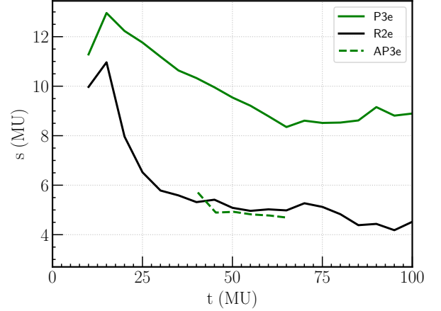
Figure 6. Time evolution of the hardening rates (Eq. 6) for the prograde equal mass run P3e, the retrograde equal mass run R2e and the model AP3e, in which the CoM of the equal mass, prograde binary is fixed at the centre of the stellar distribution. If the binary is anchored in the centre, its hardening rate gets very similar to that of the retrograde run.
