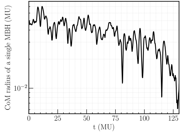
Figure 7. Displacement from the centre of the stellar distribution of a single MBH initialized by manually merging the binary in run P2e. Time t = 0 corresponds to the instant at which the MBHs in the progenitor binary are merged. The MBH gradually inspirals towards the centre of the system in response to dynamical friction, and it does no longer exhibit coherent oscillations about the system centre.
