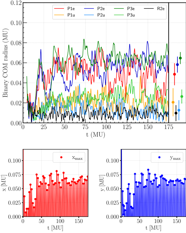
Figure 4. Upper panel: on the left is shown time evolution of the MBHB CoM radius R_b for the different runs presented in the paper; on the right, the dots indicate, for each run, the value of the binary CoM radius averaged between t = 75 and t = 175 , while the error bars show the amplitude of the Brownian wandering radius (see Tab. 2). Bottom panels: on the left is shown the time evolution of the binary CoM orbit in the x -coordinate for run P3e, the dots indicating the local maxima. The analogous is shown on the right panel for the orbit in the y -coordinate.
