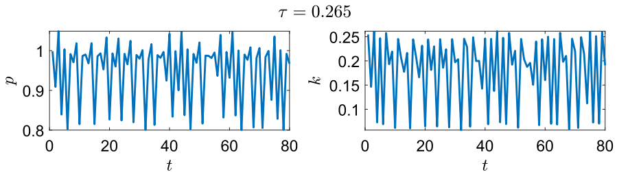
Fig. 3 Time series obtained for \theta = 1.5 and \gamma = 2 , showing chaotic endogenous oscillations. (Color figure online)
