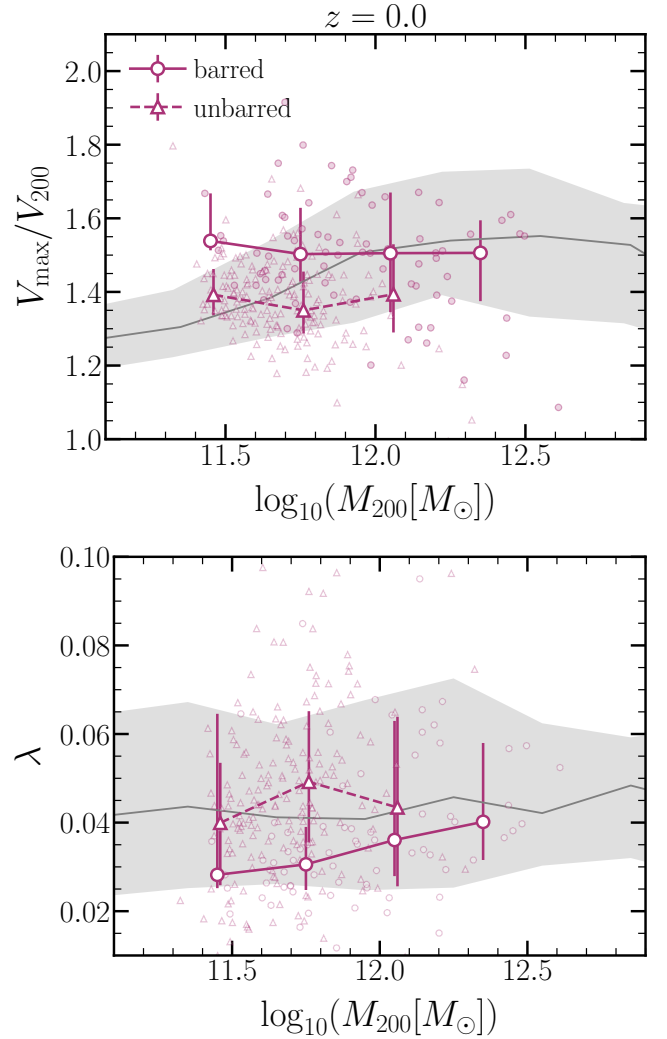
Figure 12. Top panel: V_{\max}/V_{200} - M_{200} relation at z = 0 Bottom panel: \lambda - M_{200} relation where the halo spin parameter \lambda = |\vec{J}|/(\sqrt{2}M_{200}V_{200}r_{200}) . Medians are calculated in halo mass bins with more than 5 galaxies and error bars represent the 20 th and 80 th percentiles of each distribution. Grey shaded regions and solid lines represent the 20 th and 80 th percentiles and the median for all the central TNG50 galaxies, respectively. Haloes hosting barred galaxies are likely to have higher V_{\max}/V_{200} ratios (more concentrated) with smaller spins than those populated by unbarred galaxies.
