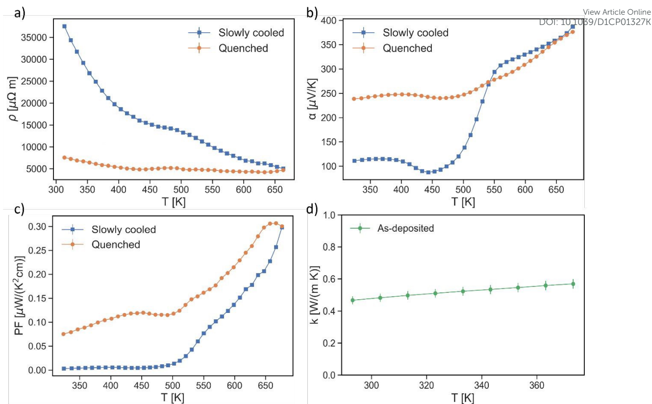
Figure 3. Electrical resistivity \rho (a), absolute Seebeck coefficient \alpha (b) and Power Factor PF (c) for spin-coated CZTS thin films. A sample after slow cooling (blue, squared markers), initially in an ordered state, and a sample after quenching from a 350 °C post-annealing (orange, circular markers), in a disordered state, have been measured. d) Thermal conductivity ( k ) for the as-deposited spin-coated sample.
