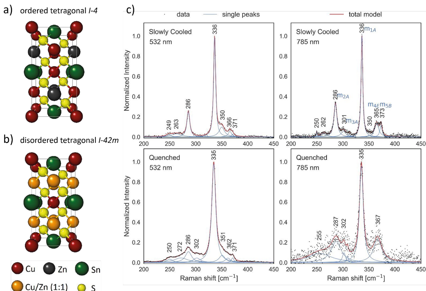
Figure 2. Crystal structures of tetragonal ordered kesterite, s.g. I-4 (a), and of tetragonal disordered, s.g. I-42m (b), involving a randomization of Cu^{+} and Zn^{2+} cations in the intermediate planes ( 2c and 2d Wyckoff positions in the ordered becoming a unique 4d site in disordered). c) Near-resonant Raman spectroscopy and peak fitting using Lorentzian curves. A sample slowly cooled after the thermal treatment and another quenched from a 350^{\circ}C post-annealing are shown, both measured with excitation wavelengths of 532 nm and 785 nm. Intensities are normalized with respect to the main mode. Mode labelling can be seen in the upper right quadrant.
