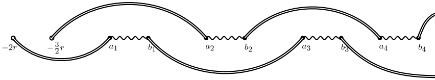
FIG. 3. Graphical representation of I_t^{(3)}(\varphi) (see (4.7)) when \varphi = g_r is the heat kernel; see (4.13). More specifically, we represent the term m = 4 in the series in (4.7). Double solid lines from b_{i-2} to a_i are assigned weights (a_i - b_{i-2})^{-1} , while wiggly lines from a_i to b_i are assigned weights G_\vartheta(b_i - a_i) .
