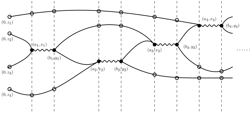
FIG. 2. Graphical representation of the kernel \mathcal{K}_1^{(4)}(z_1, z_2, z_3, z_4) for the fourth moment, see (2.16). The solid-curved and wiggly lines are assigned the same weights as in Figure 1. The hollow circles on the vertical dashed lines are where we apply the Chapman–Kolmogorov decomposition (see also Remark 2.6).
