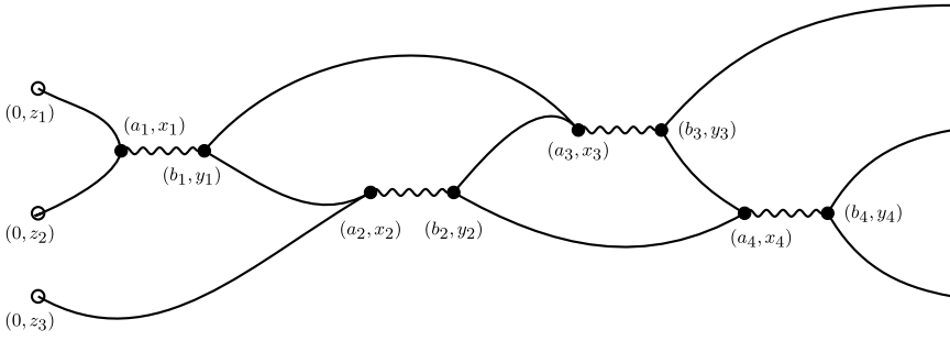
FIG. 1. Graphical representation of the kernel K_t^{(3)}(z_1, z_2, z_3) for the centered third moment, see (2.9)–(2.11). Solid-curved lines from (b, y) to (a, x) are assigned weights g_{\frac{a-b}{2}}(x - y) , while wiggly lines from (a, x) to (b, y) are assigned weights G_\vartheta(b - a)g_{\frac{b-a}{4}}(y - x) .
