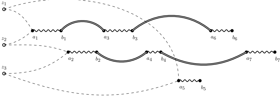
FIG. 5. Graphical representation of the term m = 7 in the series (4.37), which describes K_t^{(2)}(z_1, z_2)K_t^{(2)}(z_2, z_3)K_t^{(2)}(z_1, z_3) , see (4.36). Pairs of dashed lines from z_i, z_j to an a are assigned total weight g_a(z_i - z_j) ; double solid lines from b_{i-2} to a_i are assigned weight (a_i - b_{i-2})^{-1} ; wiggly lines from a_i to b_i are assigned weight G_\vartheta(b_i - a_i) . Referring to (4.37), we have \ell = 5 and \text{prev}(6) = 3, \text{prev}(7) = 4 .
