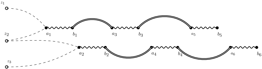
FIG. 4. Graphical representation of the term m = 6 in the series (4.34), which represents K_t^{(2)}(z_1, z_2)K_t^{(2)}(z_2, z_3) . The total weight of the dashed lines from z_1 and z_2 to a_1 is assigned weight g_{a_1}(z_2 - z_1) , and the total weight of the dashed lines from z_2 and z_3 to a_2 is assigned weight g_{a_2}(z_3 - z_2) ; a double solid line from b_{i-2} to an a_i is assigned weight (a_i - b_{i-2})^{-1} ; a wiggle line from an a_i to b_i is assigned weight G_{\vartheta}(b_i - a_i) .
