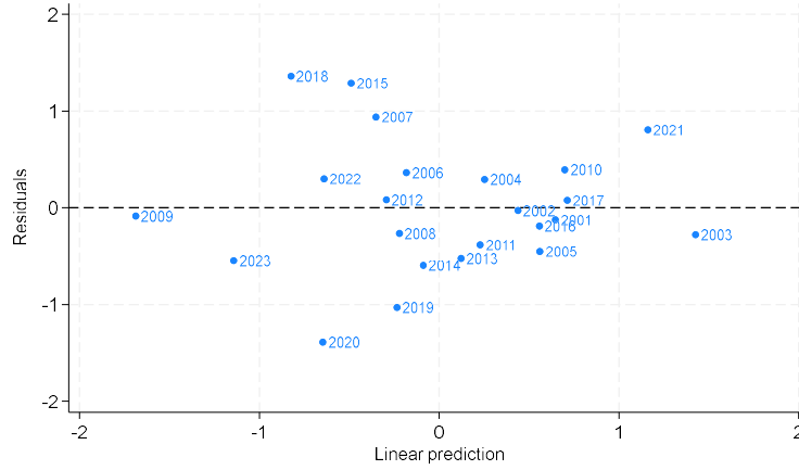
Figure 2: Residual-fitted value plot
