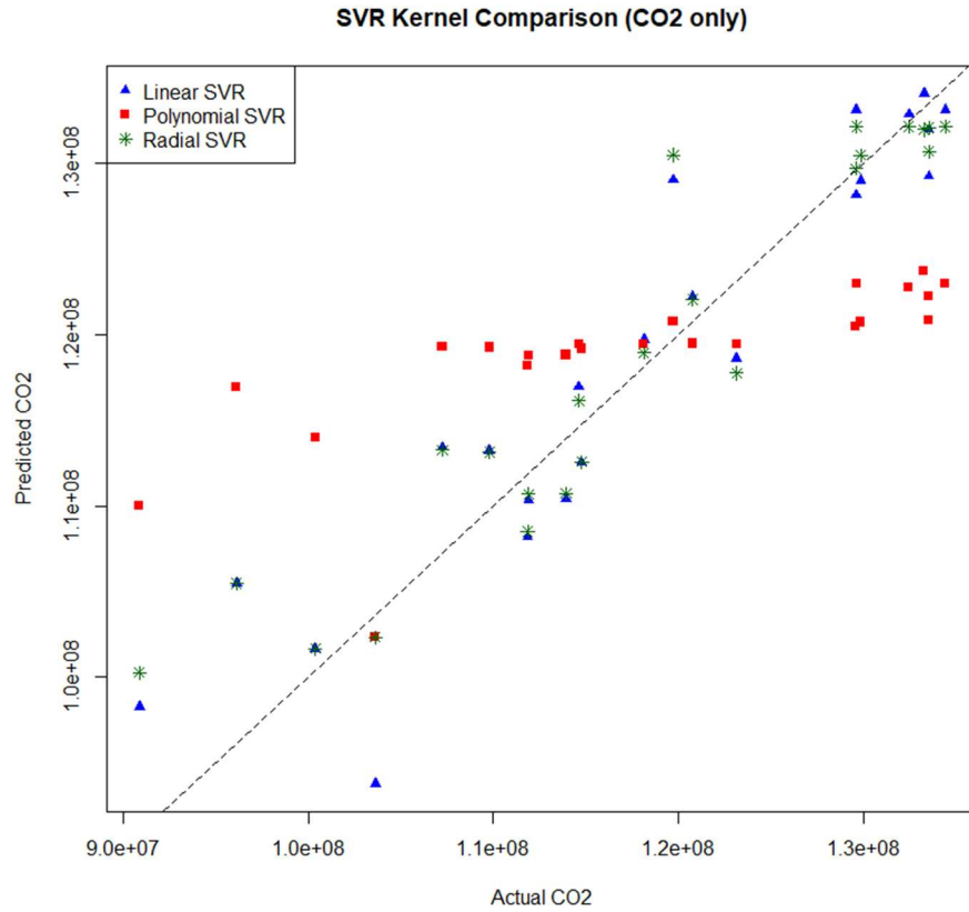
Figure A-2: SVR kernel comparison
