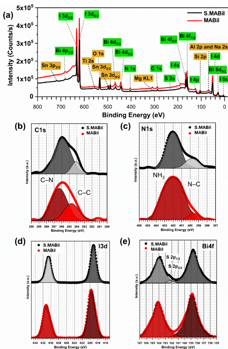
Figure 2. (a) XPS survey spectra of the sulfur-doped S.MABiI and undoped MABiI films produced by drop-casting in a nitrogen-filled glovebox on soda-lime glass. XPS high-resolution core-level spectra, related to sulfur-doped S.MABiI and undoped MABiI layers produced by drop-casting in a nitrogen-filled glovebox on soda-lime glass for (b) C 1s, (c) N 1s, (d) I 3d, and (e) Bi 4f (Raw data depicted as dots, fitting with straight lines and deconvoluted peaks by curves with the filled area).
