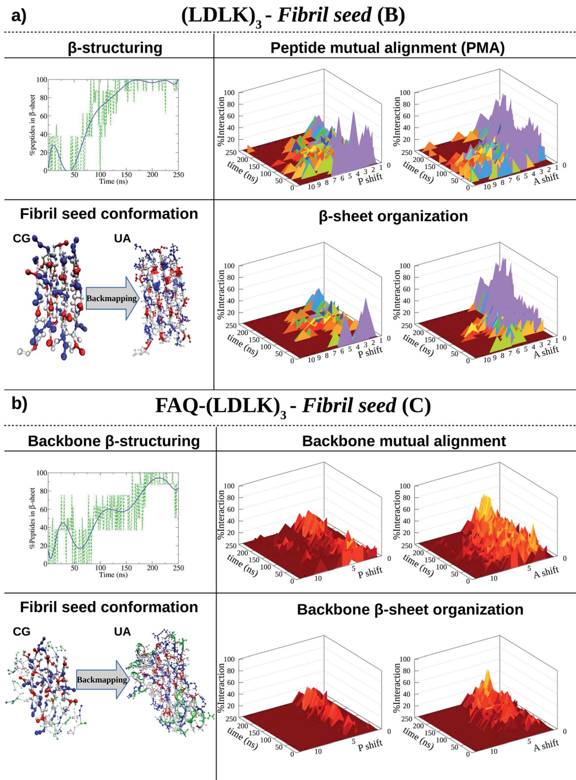
Fig. 1 Shift profiles and β-structuring propensity of (LDLK) 3 -derived SAPs. P refers to parallel alignment and A refers to anti-parallel alignment. The resulting structures from CG-MD were back-mapped and then used as starting conformations for SMD simulations. (a) In 150 ns, (LDLK) 3 SAPs aggregate into stable double-layered β-sheet structures (Morphoscanner analysis, see Section 1.7 of the ESI†), yielding strong anti-parallel alignments. Such a tendency was likely due to the electrostatic interactions among oppositely charged side chains of lysine and aspartic acid residues. (b) Alignment analysis of FAQ-(LDLK) 3 backbones showed weaker alignments in both A and P, mirrored by lower β-sheet organization. This feature was likely due to the presence of the FAQ functional motif at N-termini, which may have interfered with β-sheet formation among self-assembling backbones.
