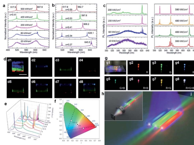
Fig. 9 Monolithic multi-color lasers based on single lateral hetero-nanobelts. (a) Power-dependent PL spectra of a CdS–CdS 0.5 Se tri-lane hetero-nanobelt. (b) Lasing spectra from CdS–CdS 0.5 Se tri-lane hetero-nanobelts with different S/Se ratios ( x ) in the middle lanes. (c) Power-dependent PL spectra of a CdS–CdS 0.5 Se lateral graded nanobelt. (d) Real-color images of a single ZnCdS 0.5 Se multi-lane nanobelt, under low pumping (d1) and above-threshold pumping (d2–d8). (e) Corresponding PL spectra acquired from panels d2 to d8. (f) Chromaticity of the lasing peaks extracted from the spectra in (e). (g1) Photograph of the mixed emission colour. (g2–g8) Photographs of the enlarged dashed-box region in (g1) when the different combinations of segments are pumped as indicated by the labels inside each figure, creating the mixed far-field emission colours red, green, blue, yellow, cyan, magenta and white. The top dots in each photograph are the direct images of laser emission, while the tails under these dots are the reflections from the substrate. (h) Schematic diagram for achieving a monolithic white laser from an individual multi-lane hetero-nanobelt. (a and b) Reproduced with permission. 45 Copyright 2012, American Chemical Society. (c) Reproduced with permission. 49 Copyright 2016, Springer. (d–h) Reproduced with permission. 15 Copyright 2015, Nature Publishing Group.
